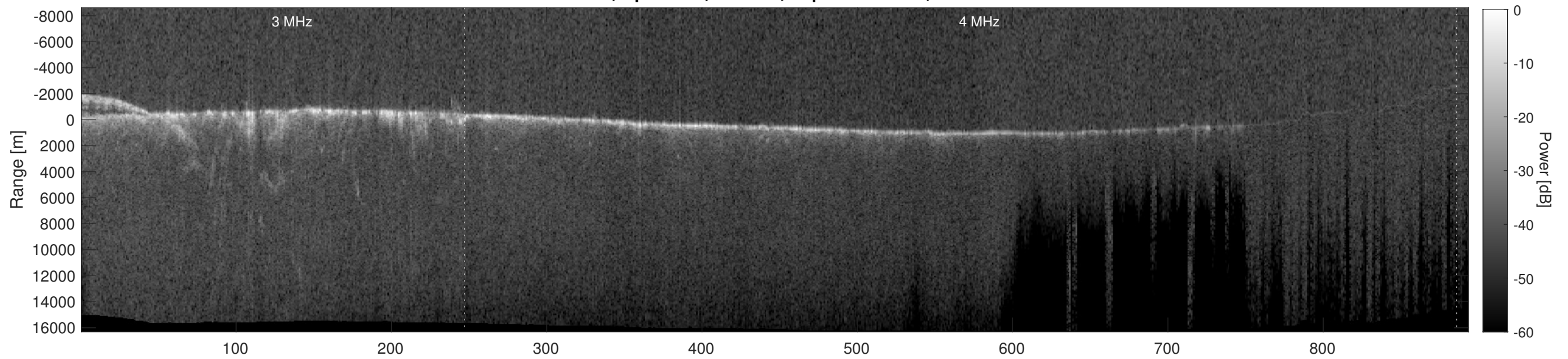
Orbit 9462, Depth-Corrected Cluttergram
