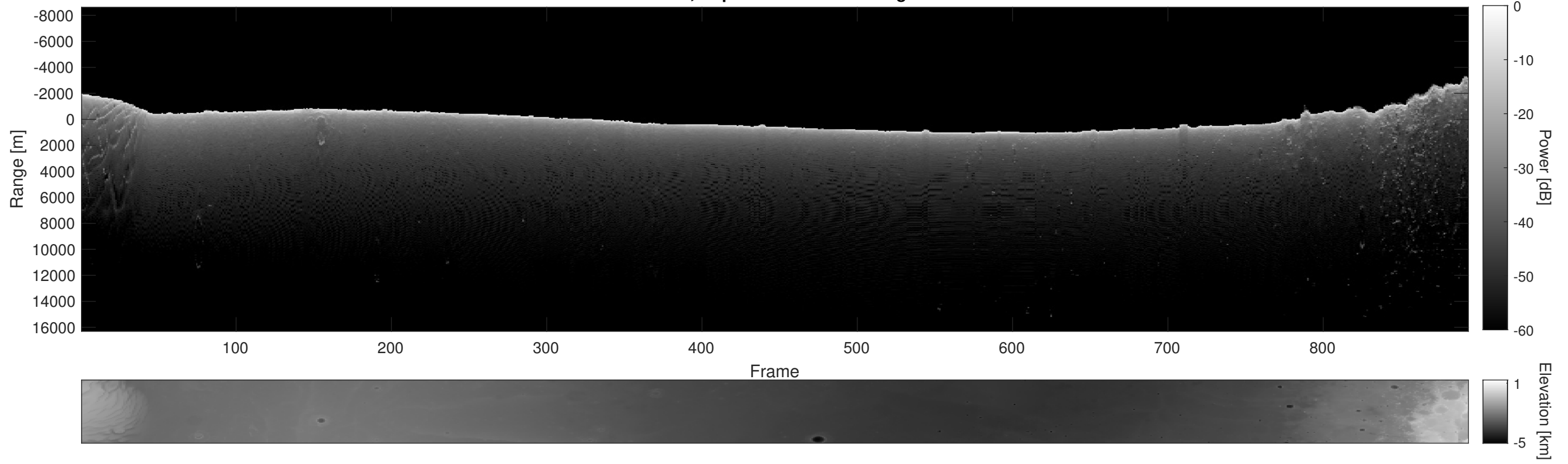
Orbit 9462, Depth-Corrected Cluttergram
