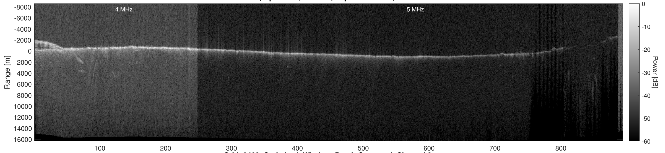
Orbit 9462, Optimized, Window, Depth-Corrected, Channel 2
