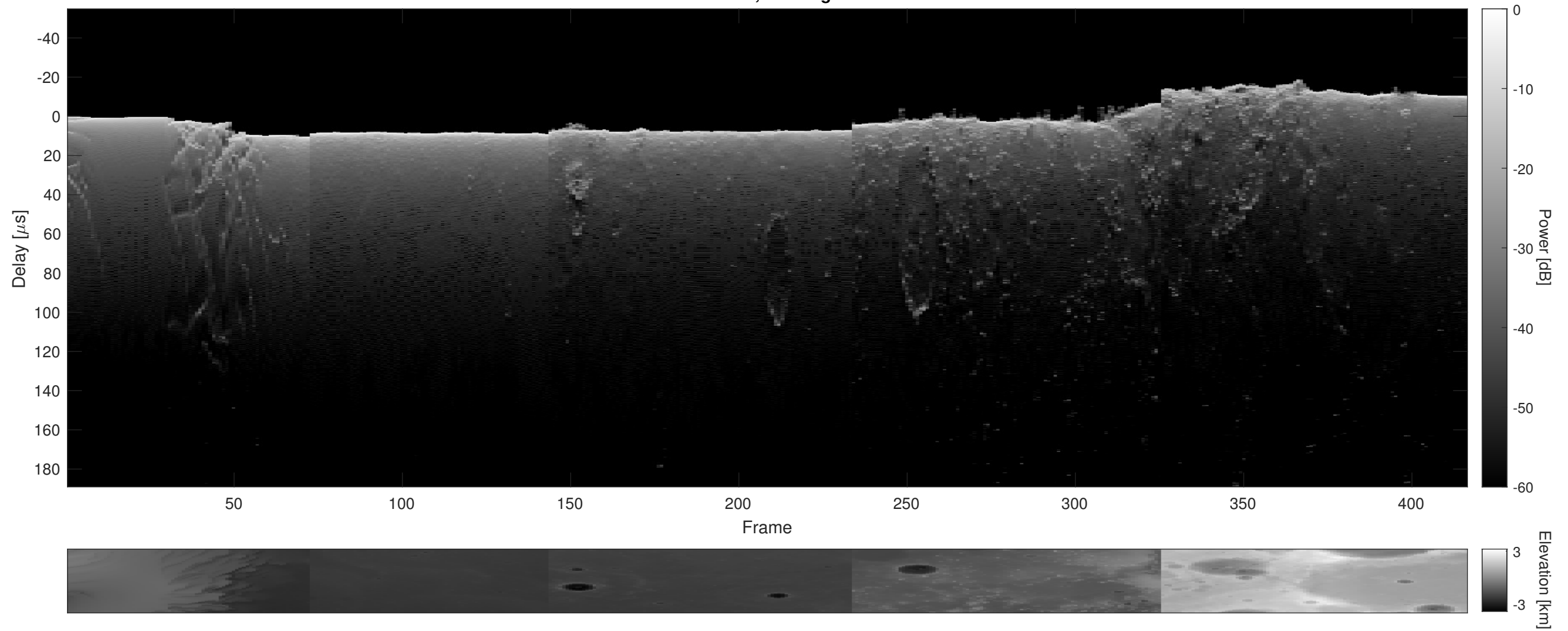
Orbit 9466, Cluttergram
