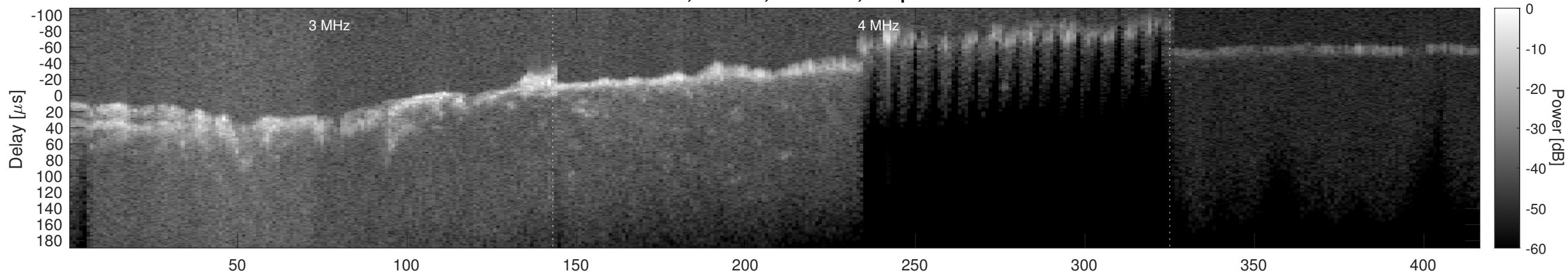
Orbit 9466, Window, Channel 2, Optimized
