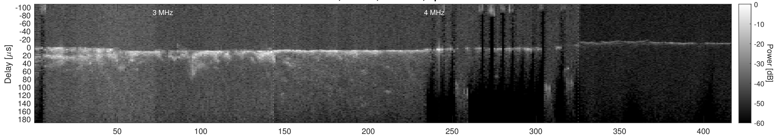
Orbit 9466, Cluttergram
