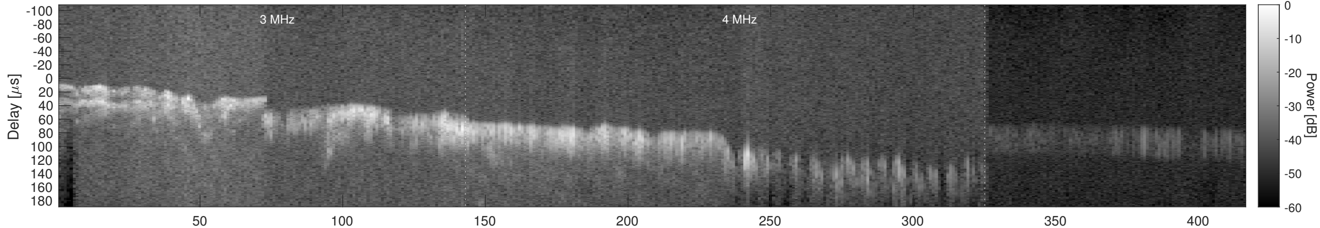
Orbit 9466, Window, Channel 2, Chapman
