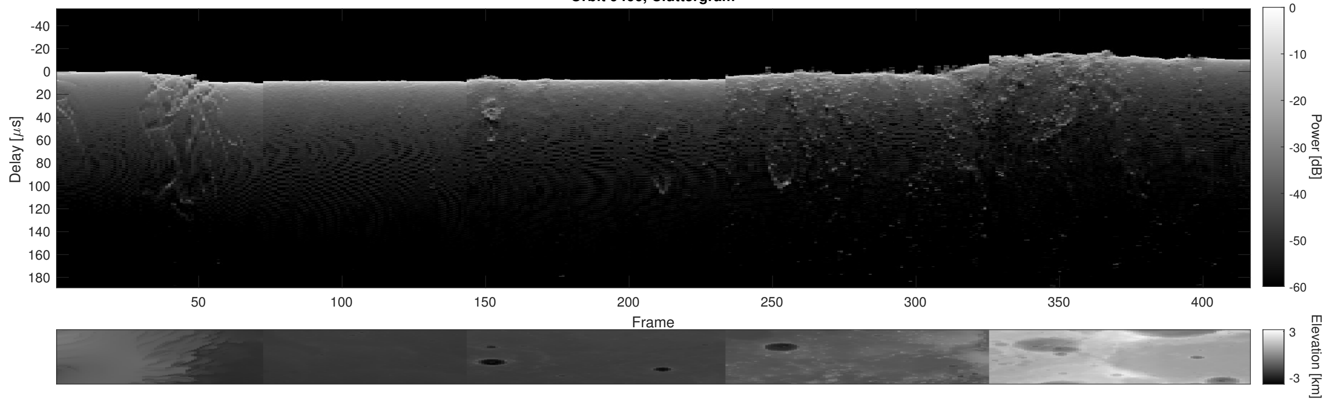
Orbit 9466, Cluttergram
