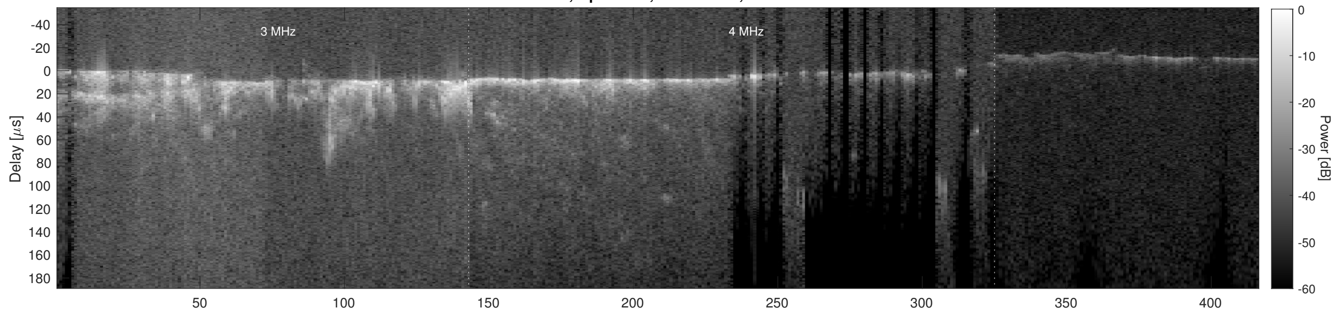
Orbit 9466, Cluttergram
