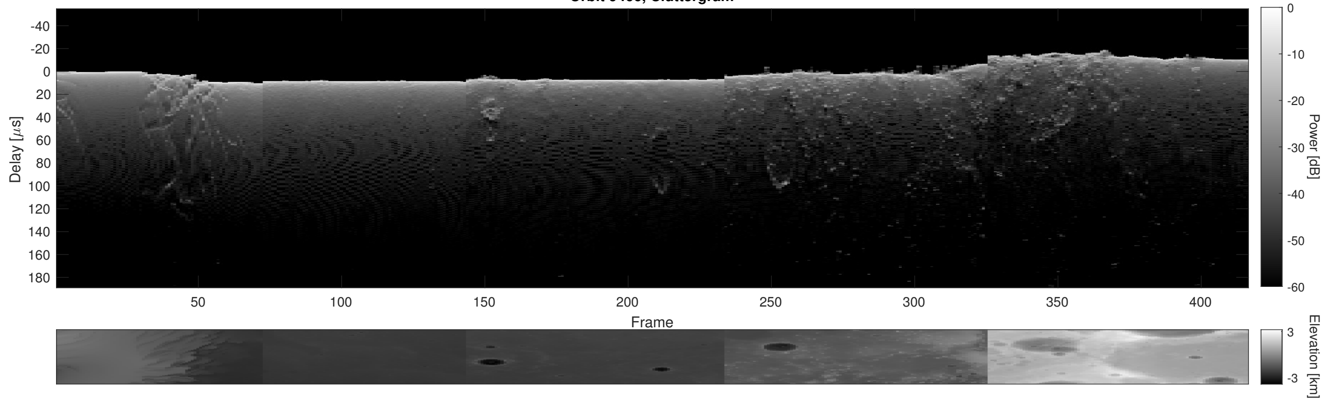
Orbit 9466, Cluttergram
