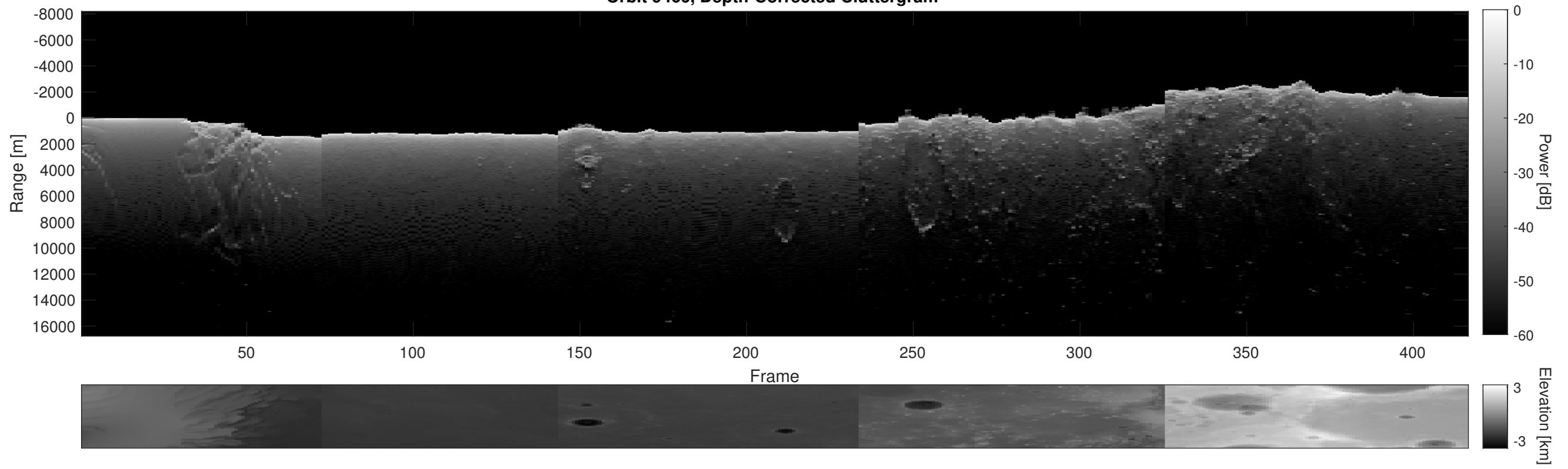
Orbit 9466, Depth-Corrected Cluttergram
