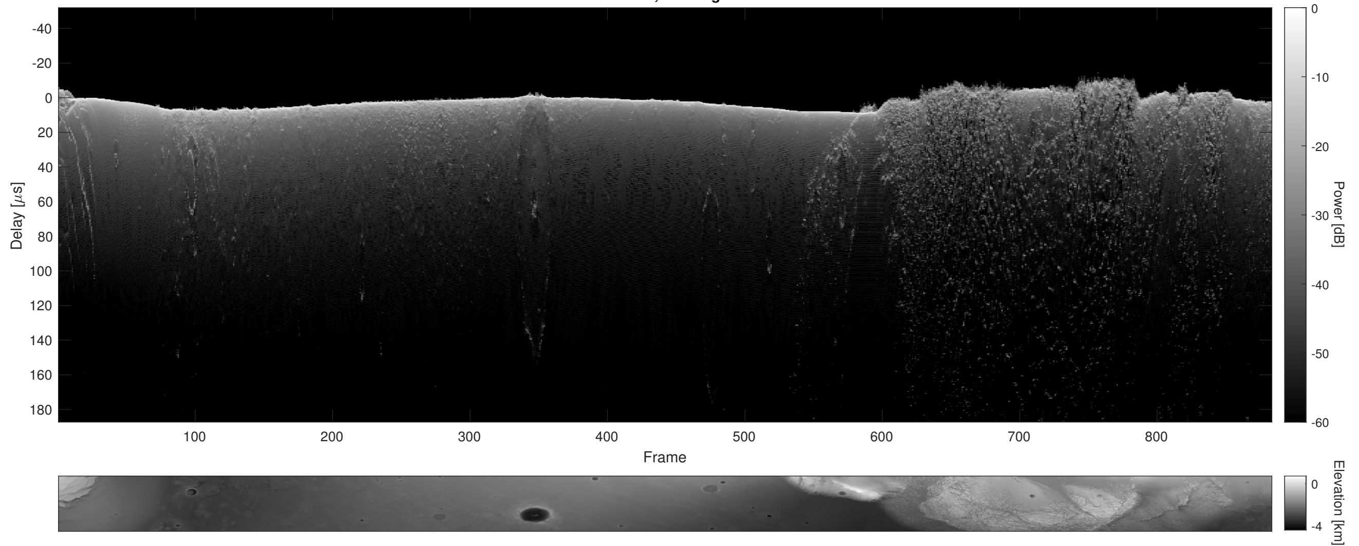
Orbit 9468, Cluttergram
