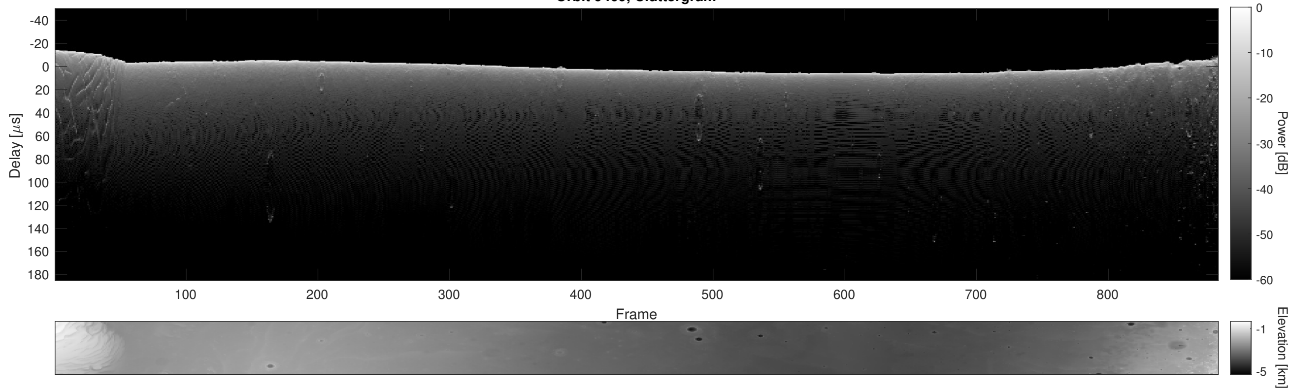
Orbit 9469, Cluttergram
