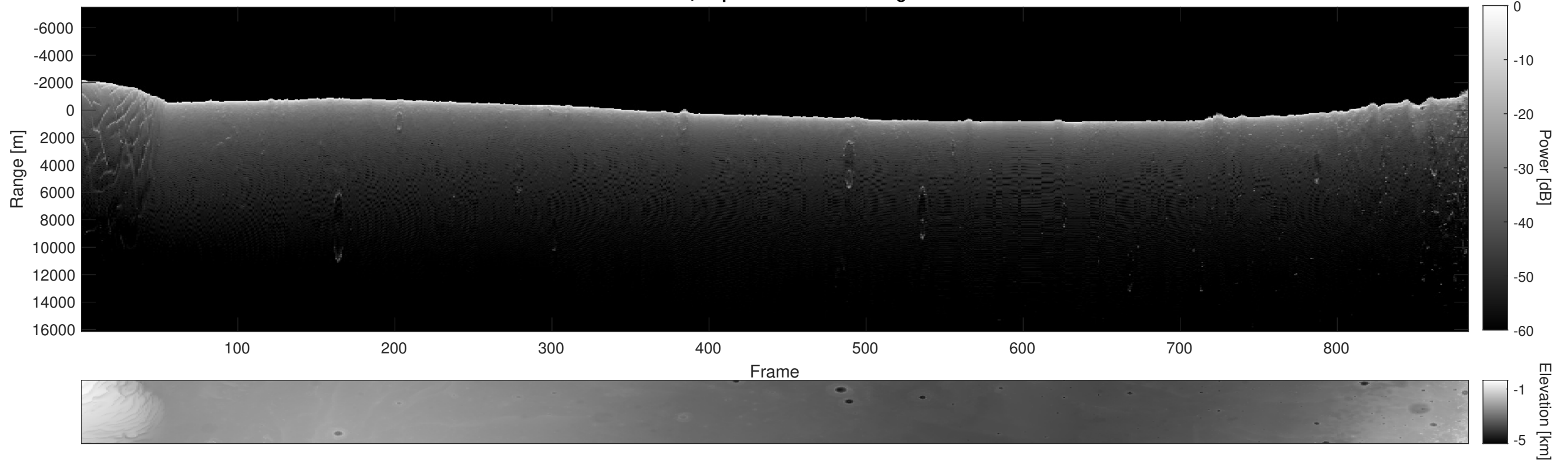
Orbit 9469, Depth-Corrected Cluttergram
