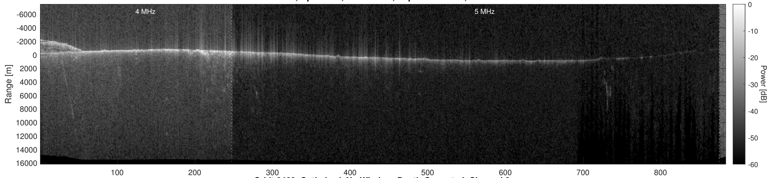
Orbit 9469, Optimized, No Window, Depth-Corrected, Channel 2
