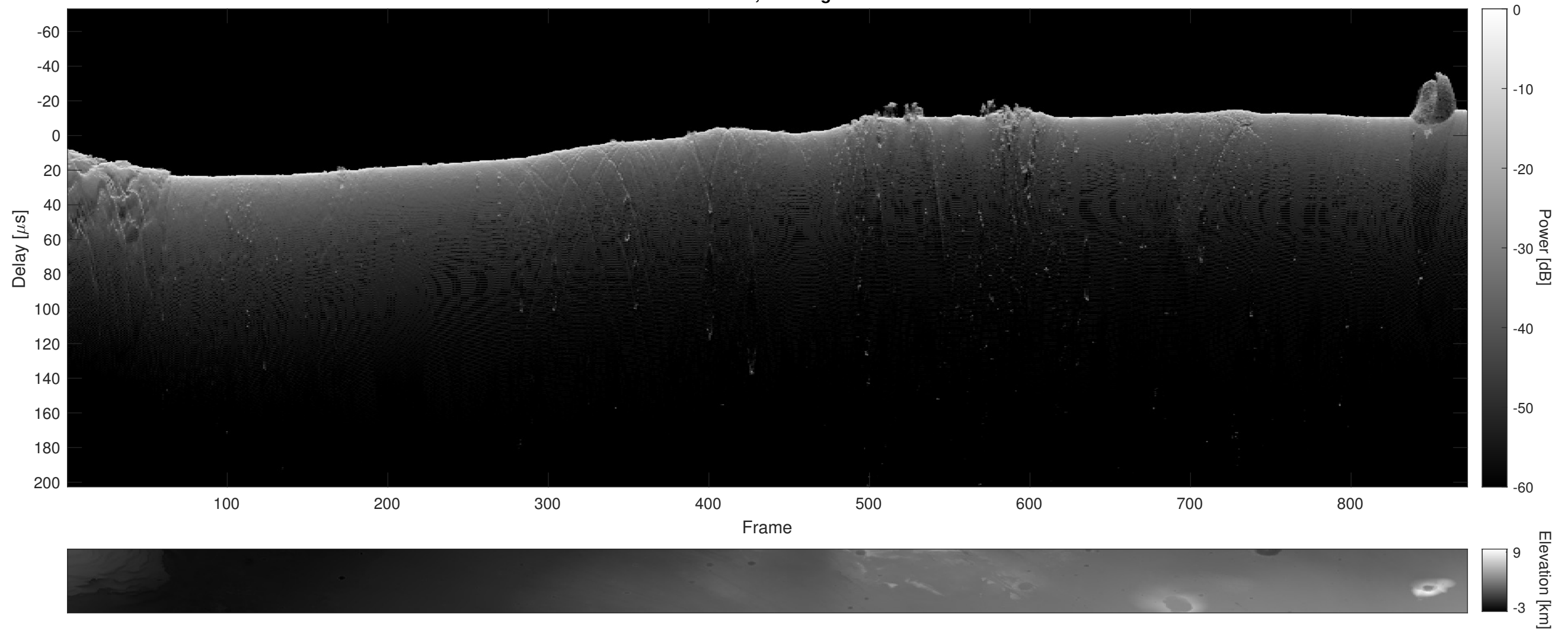
Orbit 9471, Cluttergram
