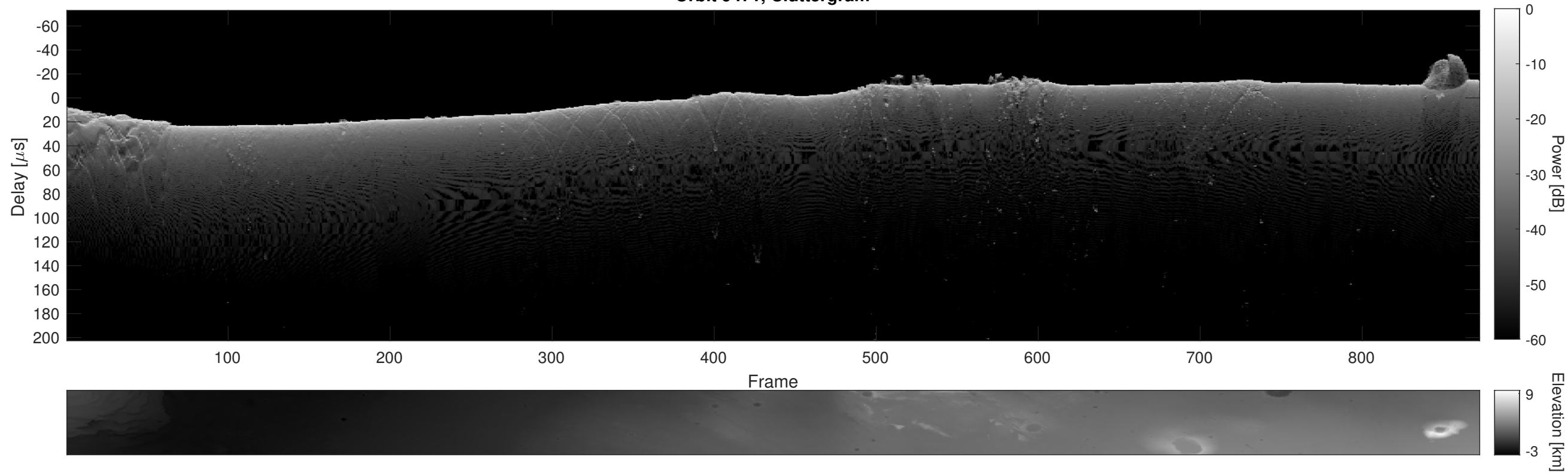
Orbit 9471, Cluttergram
