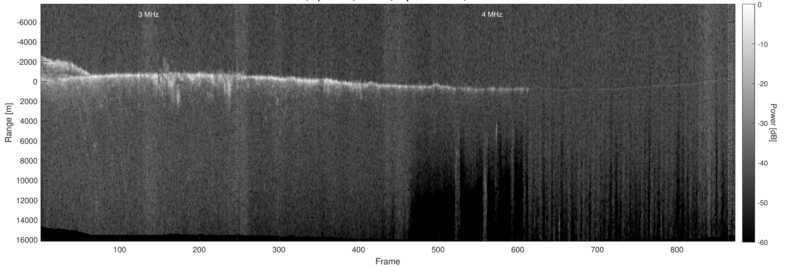
Orbit 9476, Optimized, Window, Depth-Corrected, Channel 2
