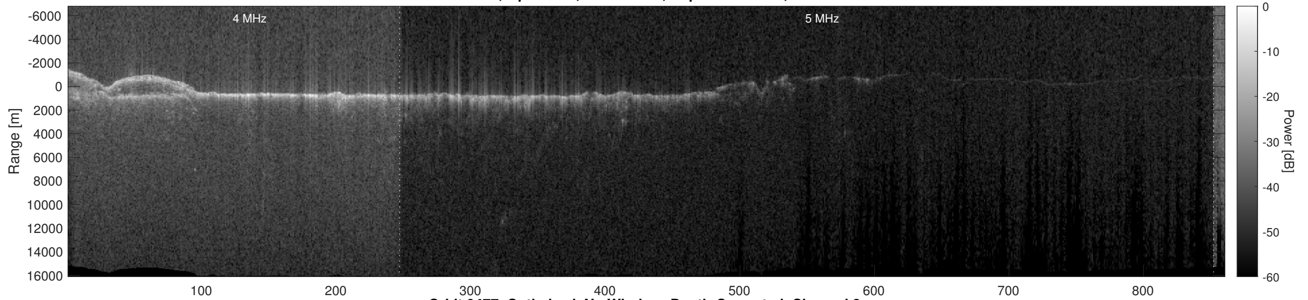
Orbit 9477, Optimized, No Window, Depth-Corrected, Channel 2
