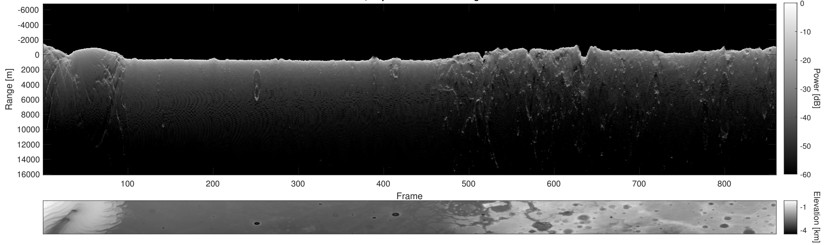
Orbit 9477, Depth-Corrected Cluttergram
