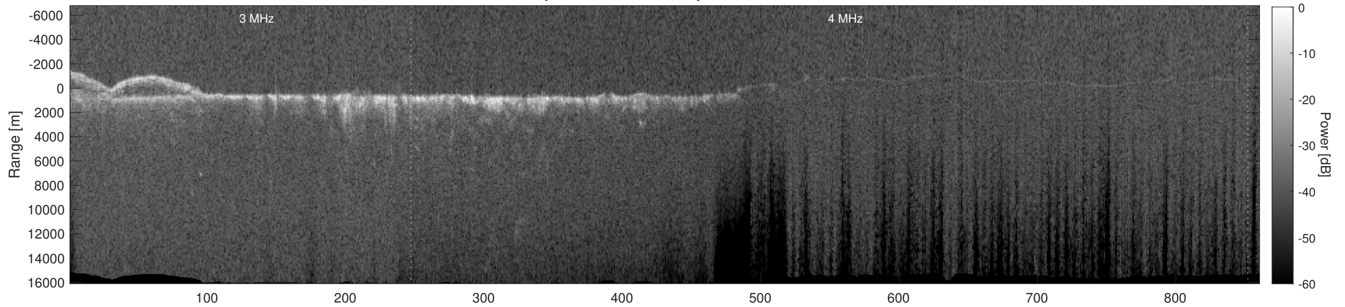
Orbit 9477, Depth-Corrected Cluttergram
