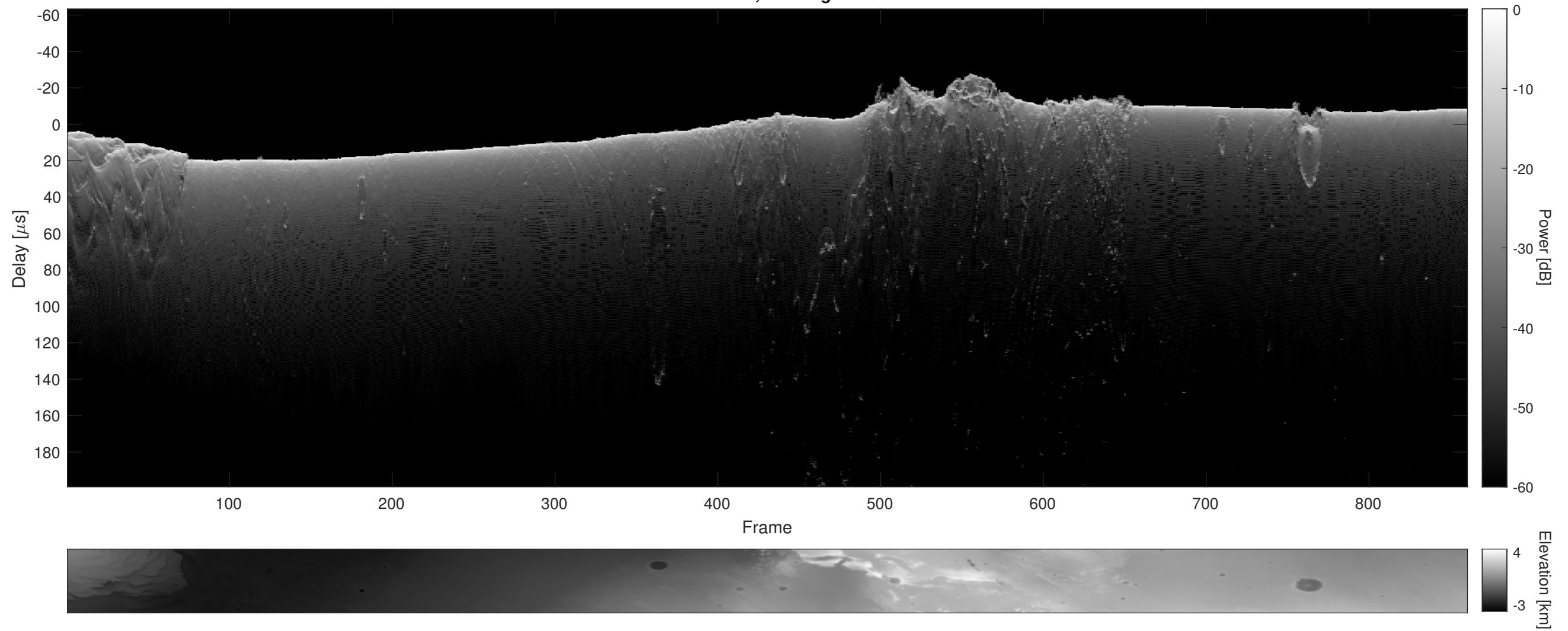
Orbit 9478, Cluttergram
