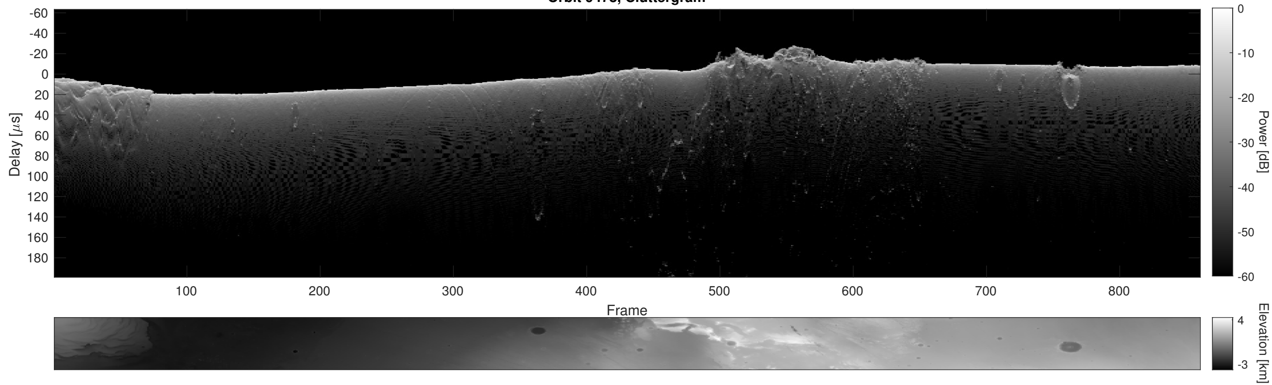
Orbit 9478, Cluttergram
