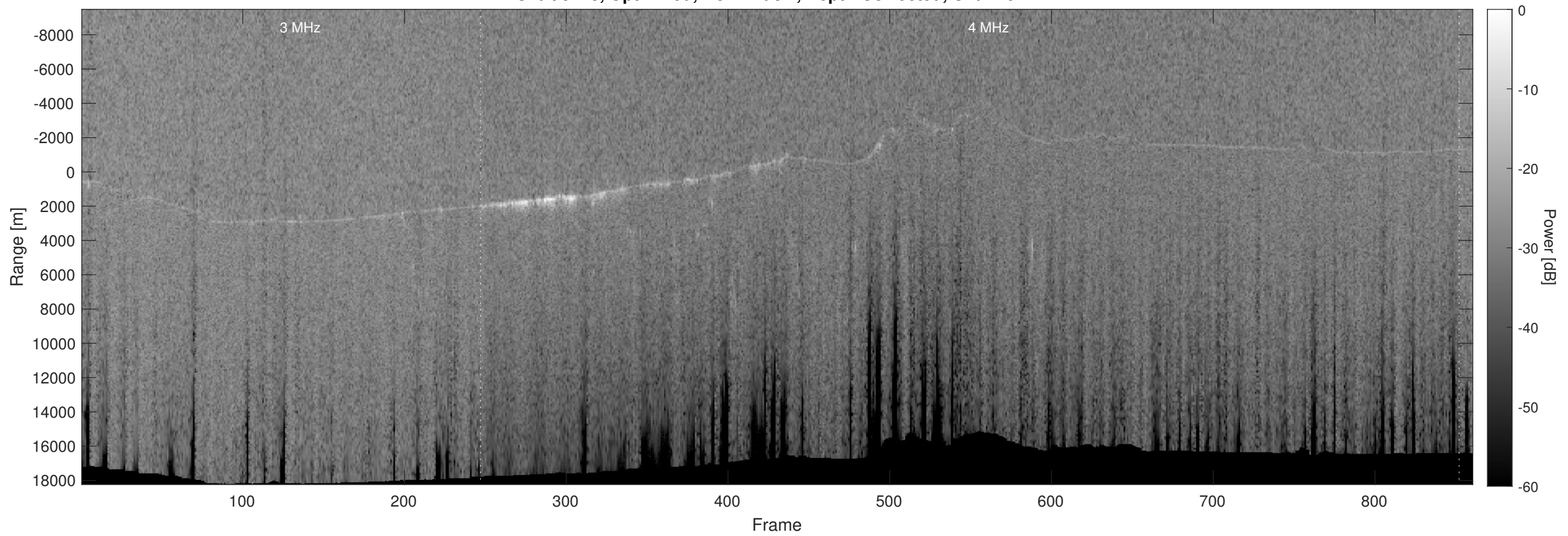
Orbit 9478, Optimized, No Window, Depth-Corrected, Channel 2
