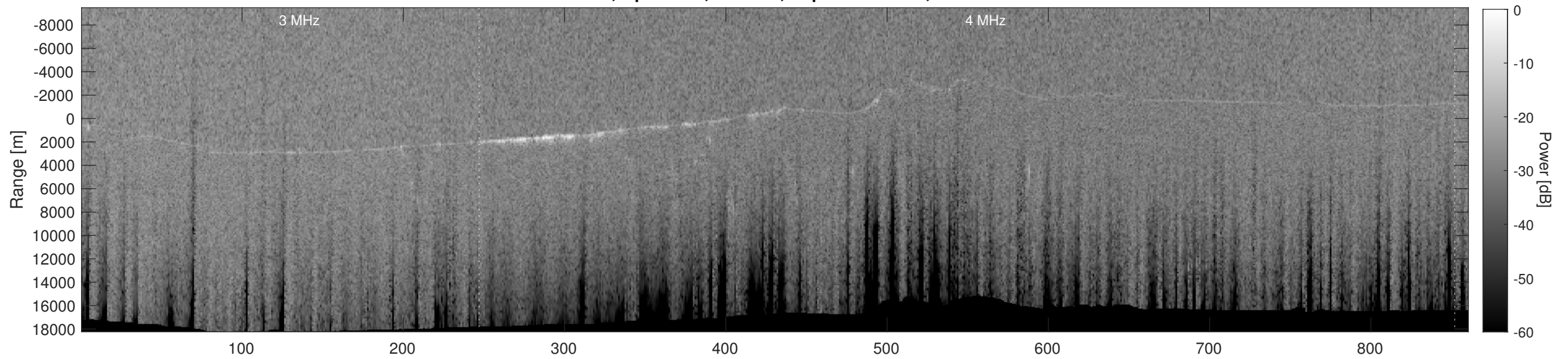
Orbit 9478, Depth-Corrected Cluttergram
