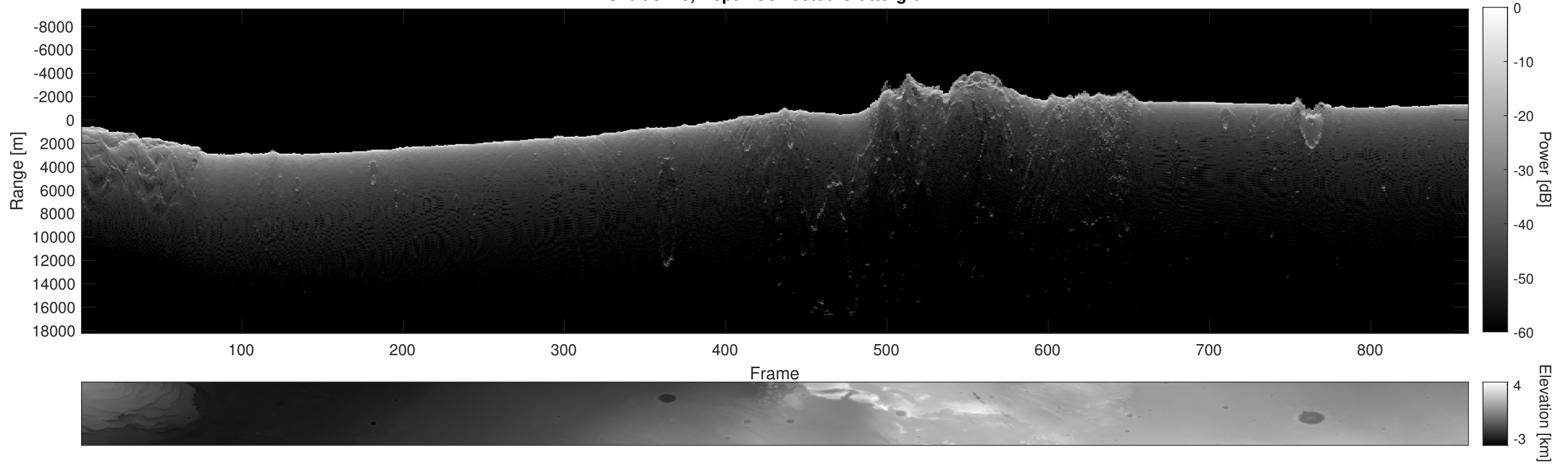
Orbit 9478, Depth-Corrected Cluttergram
