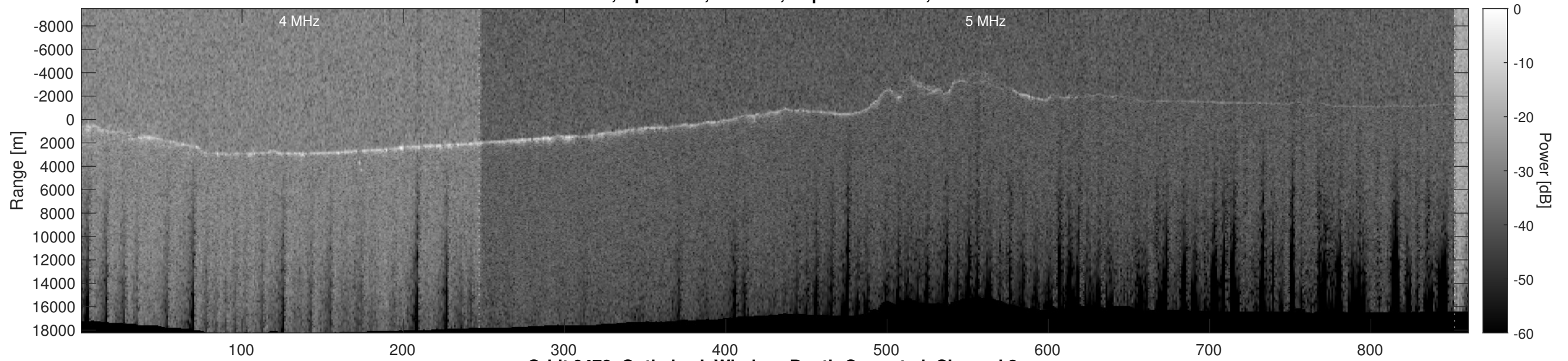
Orbit 9478, Optimized, Window, Depth-Corrected, Channel 2
