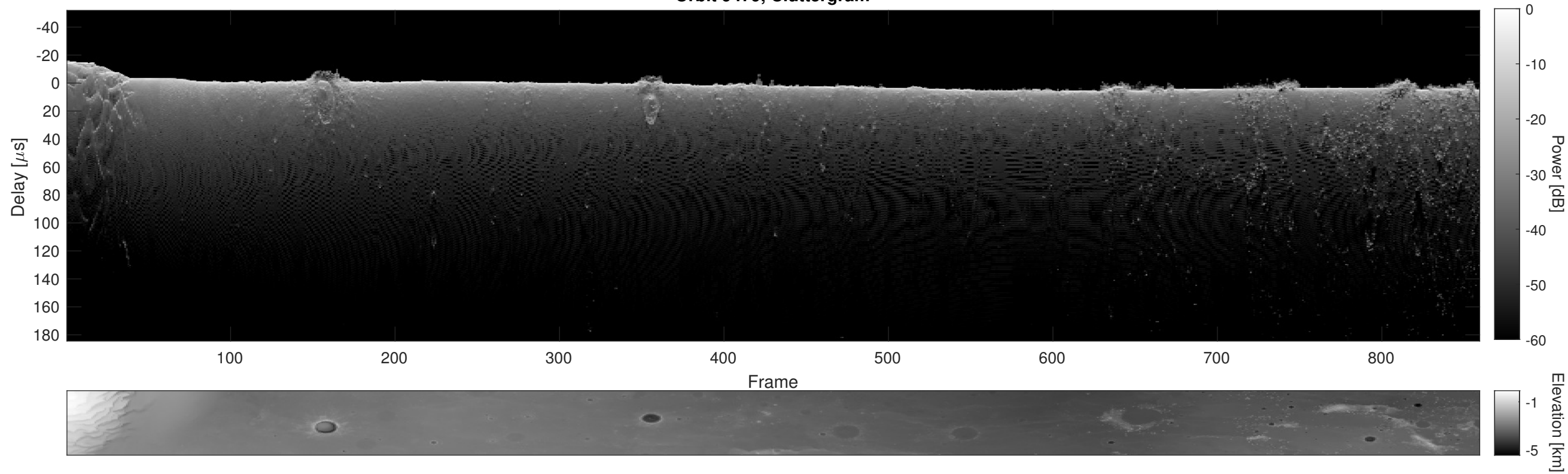
Orbit 9479, Cluttergram
