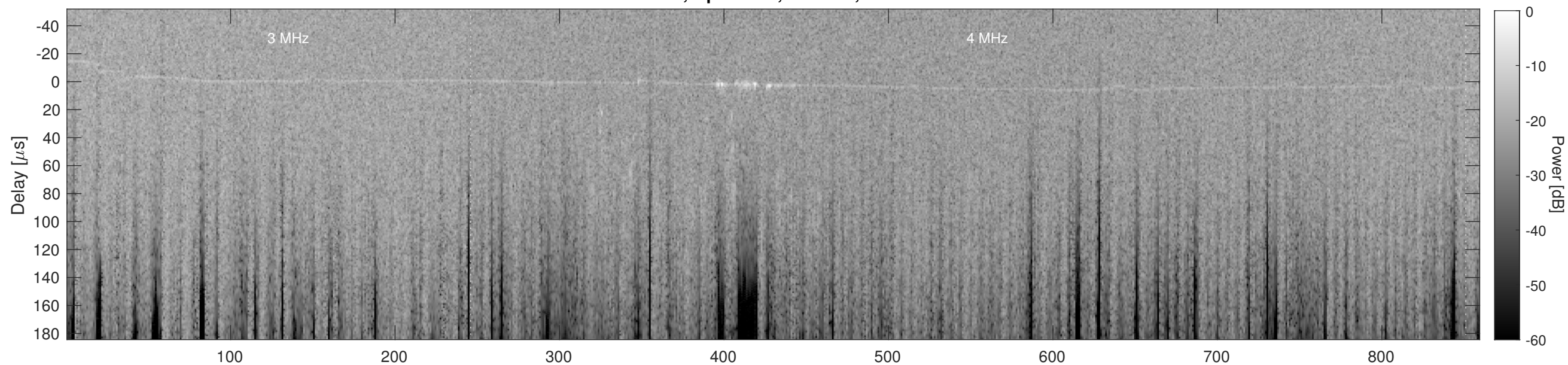
Orbit 9479, Cluttergram
