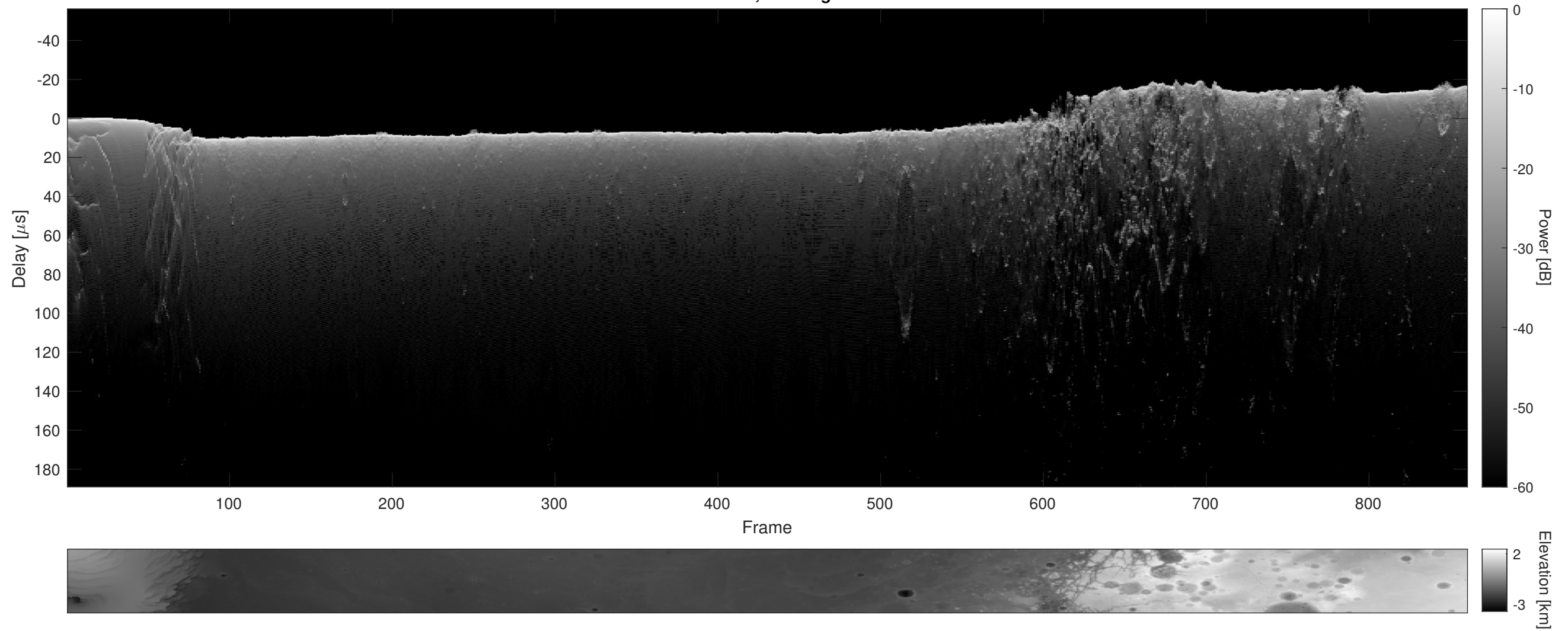
Orbit 9480, Cluttergram
