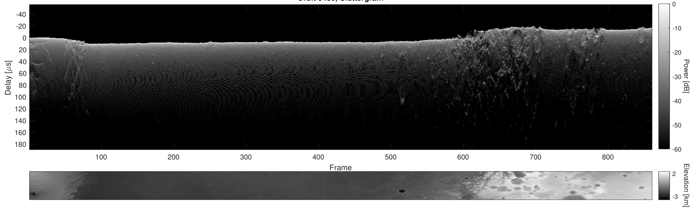
Orbit 9480, Cluttergram
