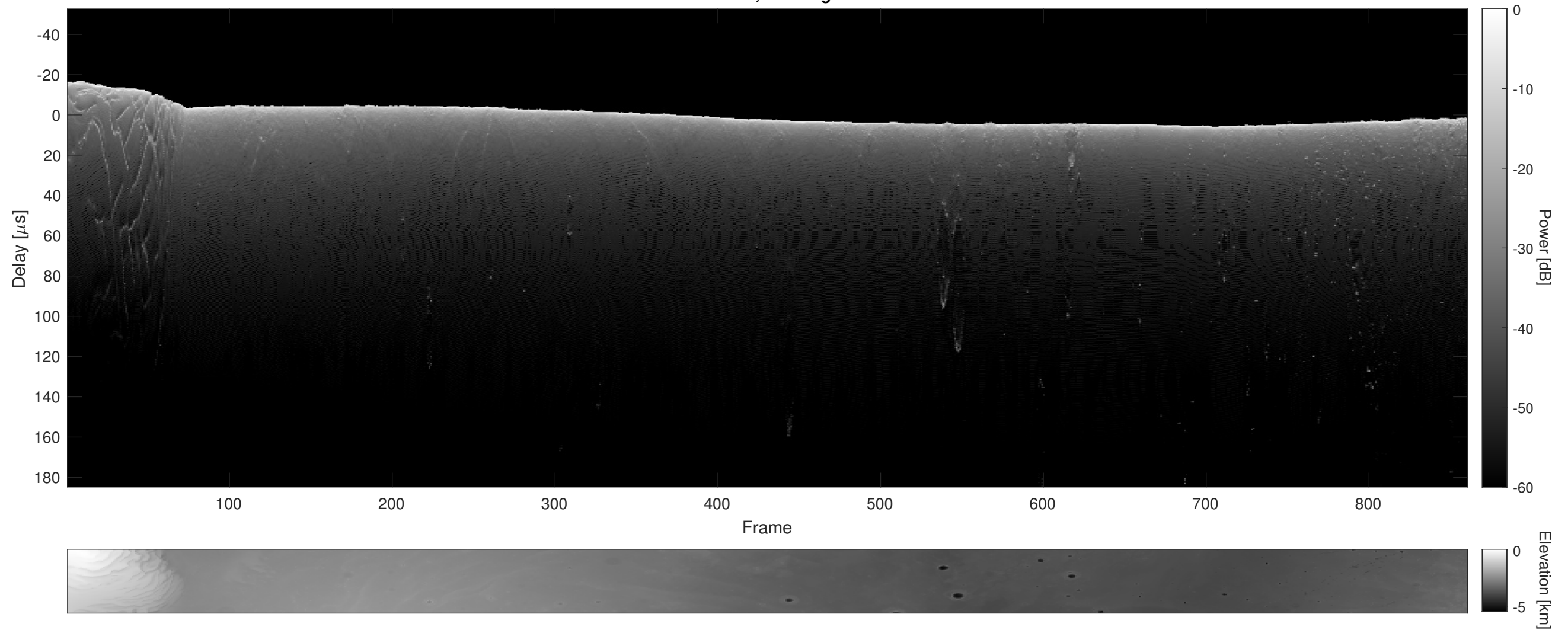
Orbit 9483, Cluttergram
