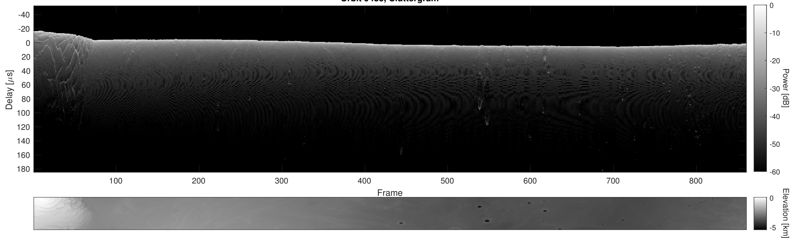
Orbit 9483, Cluttergram
