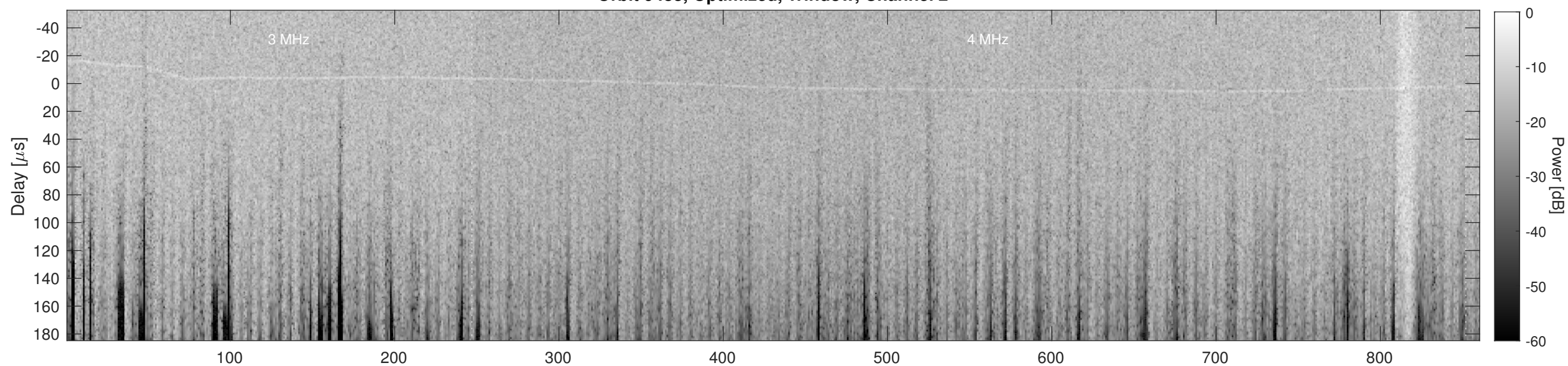
Orbit 9483, Cluttergram
