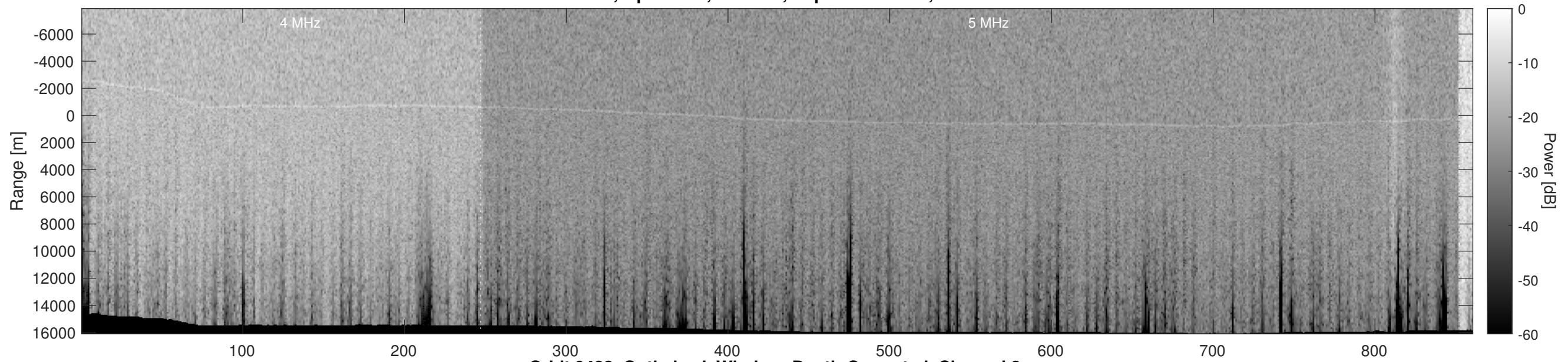
Orbit 9483, Optimized, Window, Depth-Corrected, Channel 2
