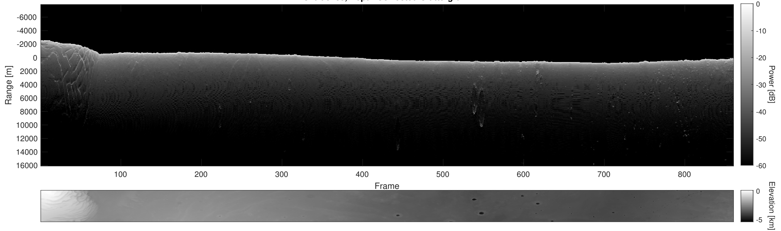
Orbit 9483, Depth-Corrected Cluttergram
