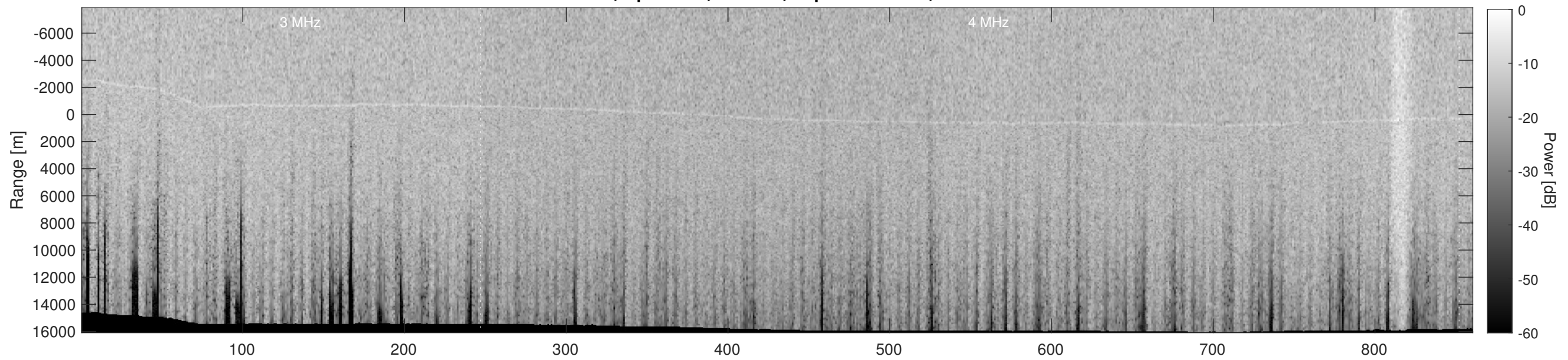
Orbit 9483, Depth-Corrected Cluttergram
