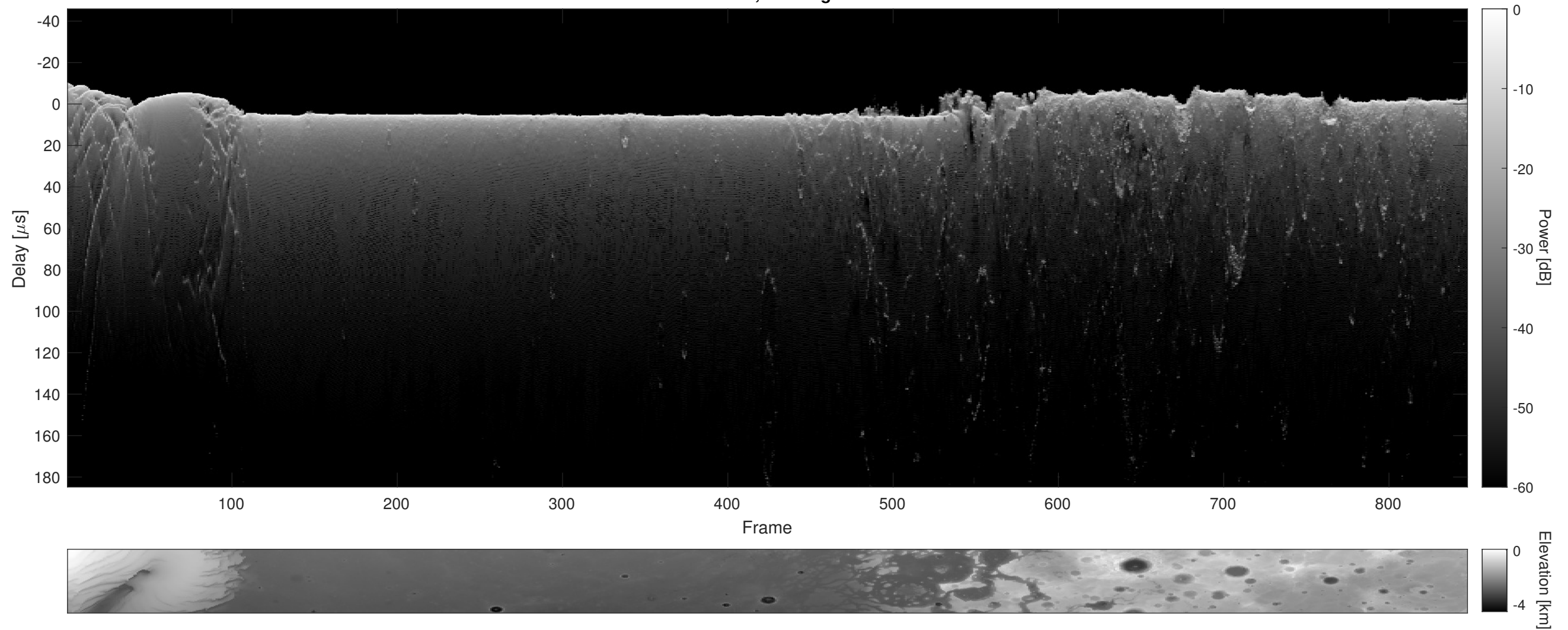
Orbit 9484, Cluttergram
