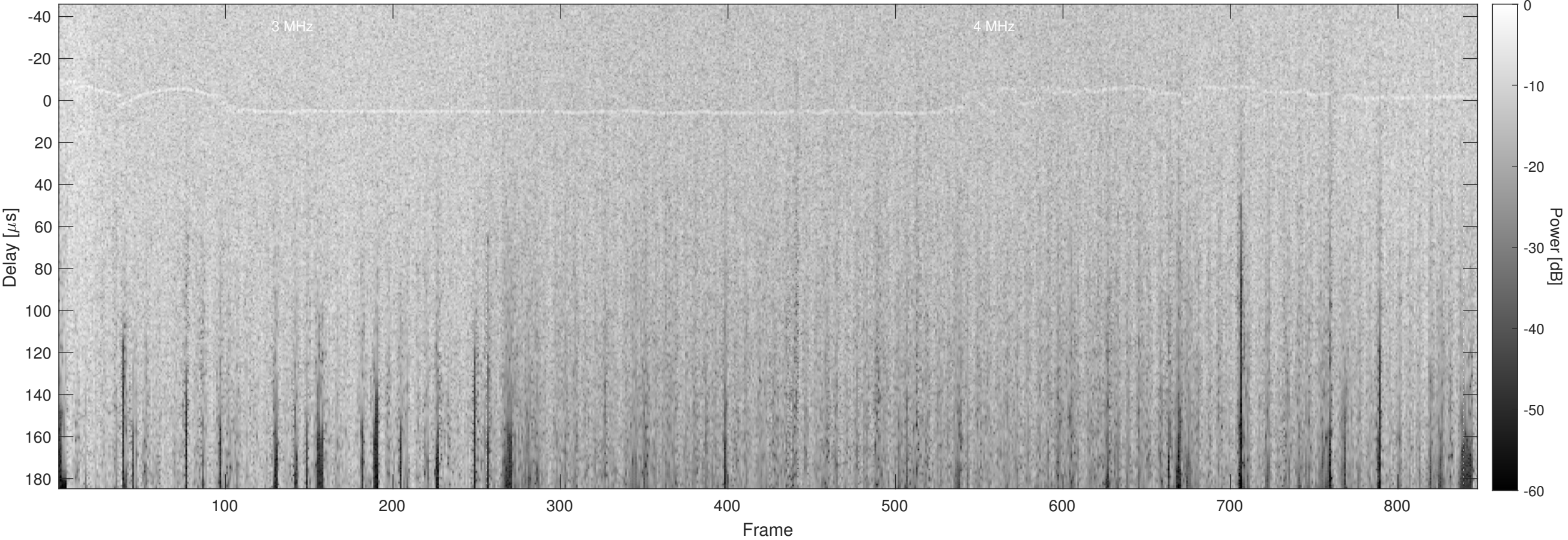
Orbit 9484, Optimized, No Window, Channel 2
