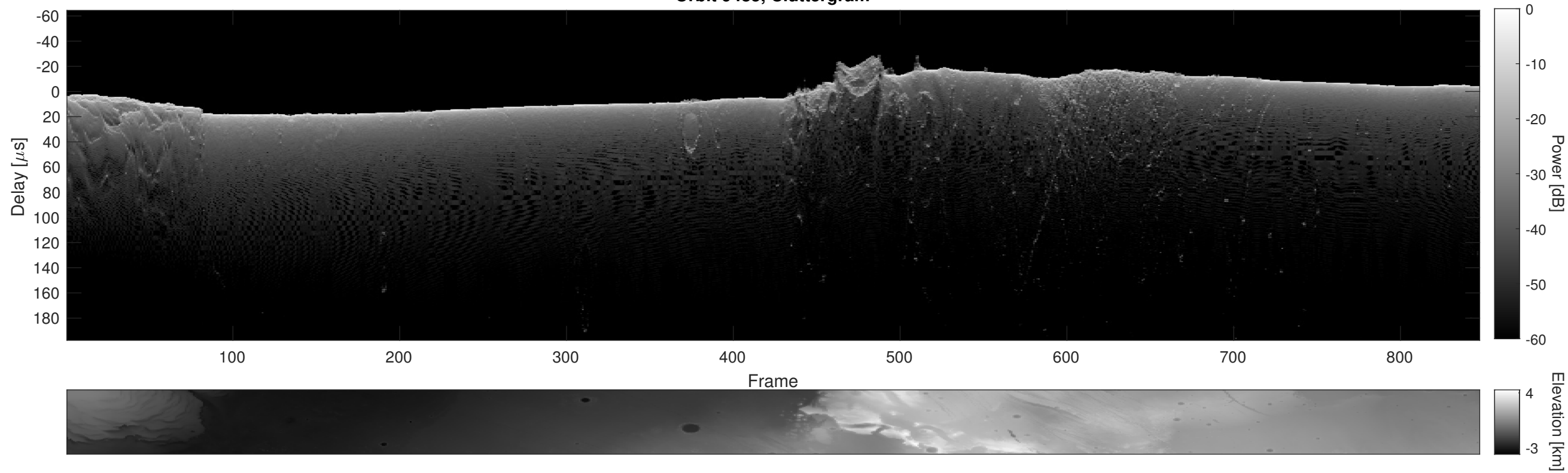
Orbit 9485, Cluttergram
