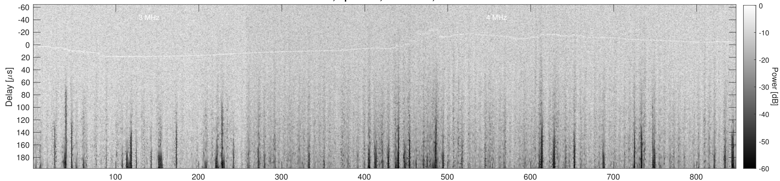
Orbit 9485, Cluttergram
