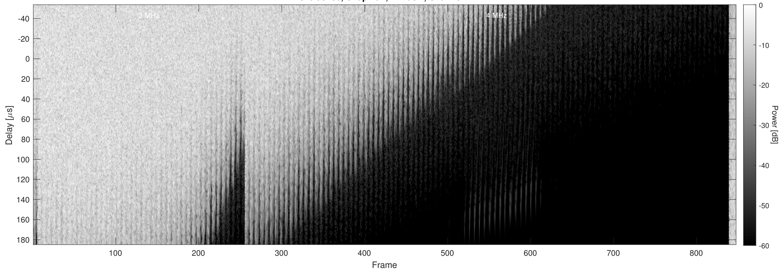
Orbit 9486, Chapman, Window, Channel 2
