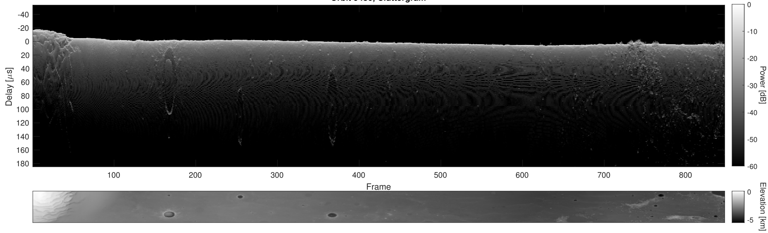
Orbit 9486, Cluttergram
