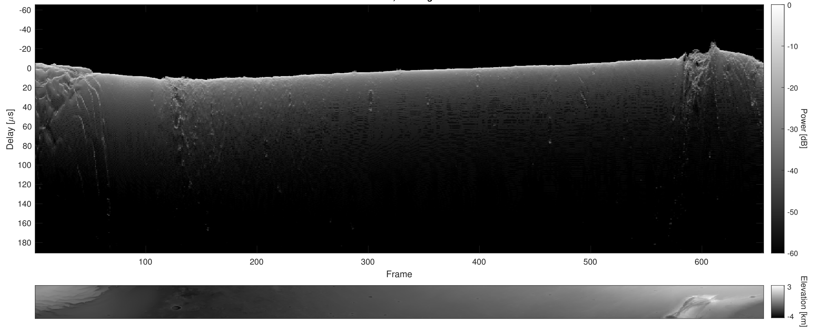
Orbit 9489, Cluttergram
