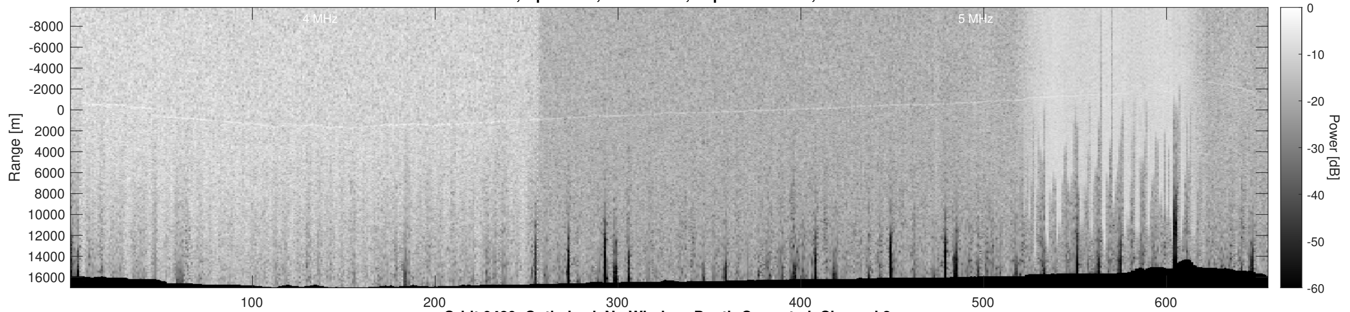
Orbit 9489, Optimized, No Window, Depth-Corrected, Channel 2
