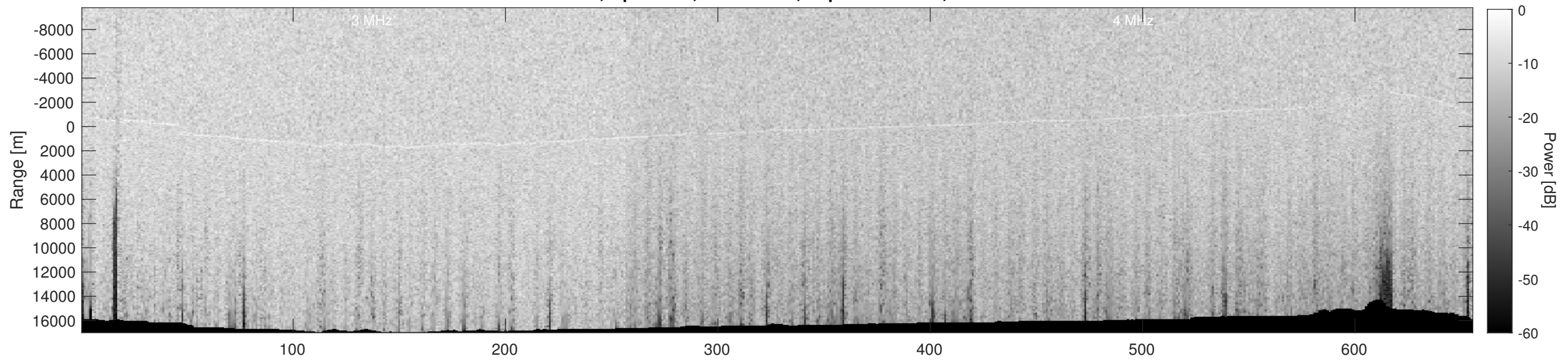
Orbit 9489, Depth-Corrected Cluttergram
