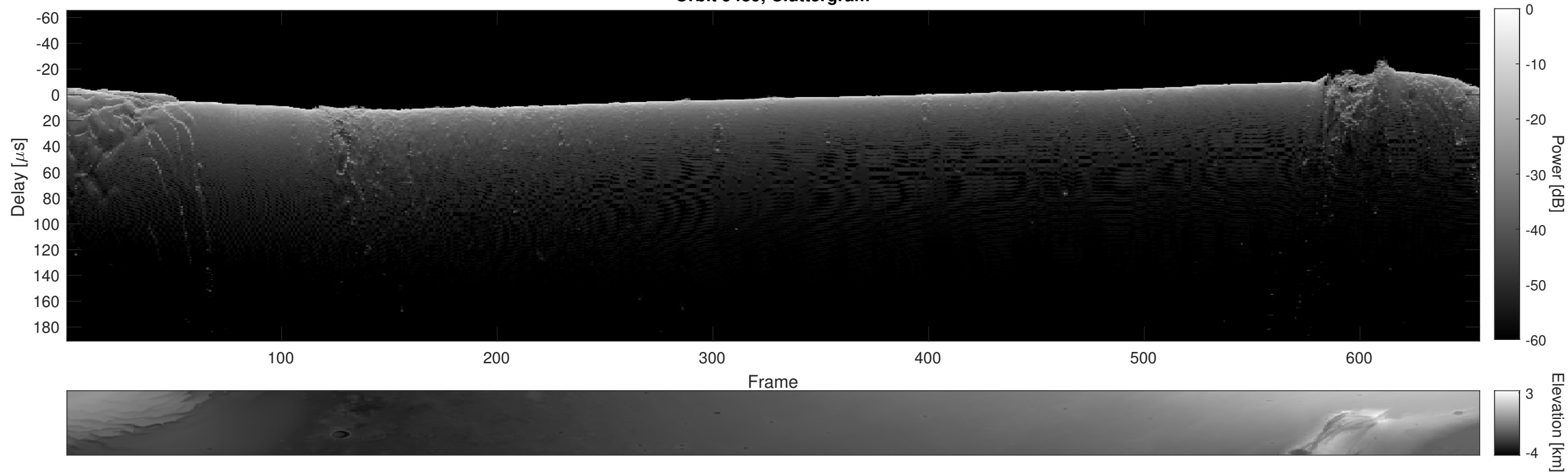
Orbit 9489, Cluttergram
