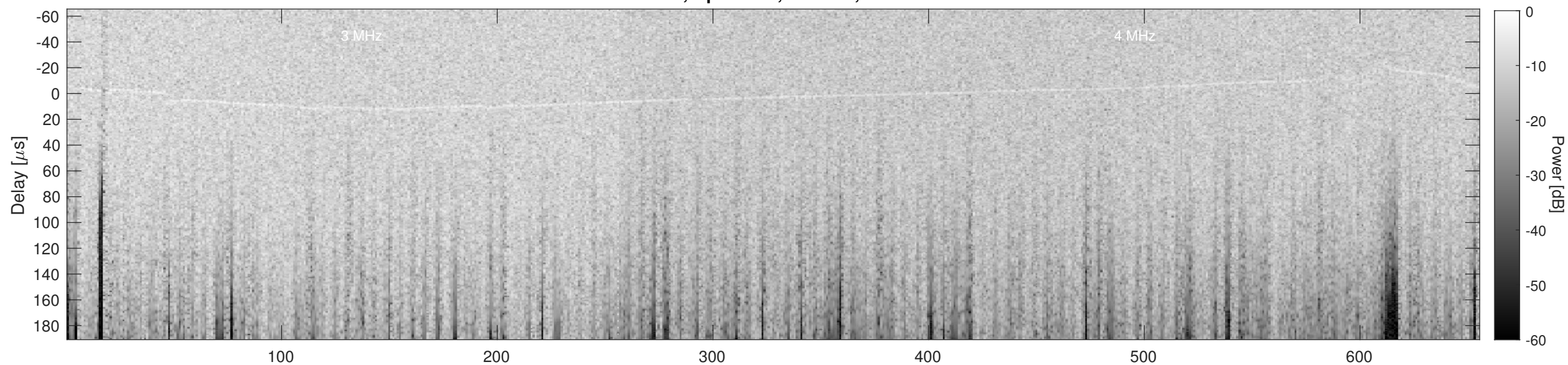
Orbit 9489, Cluttergram
