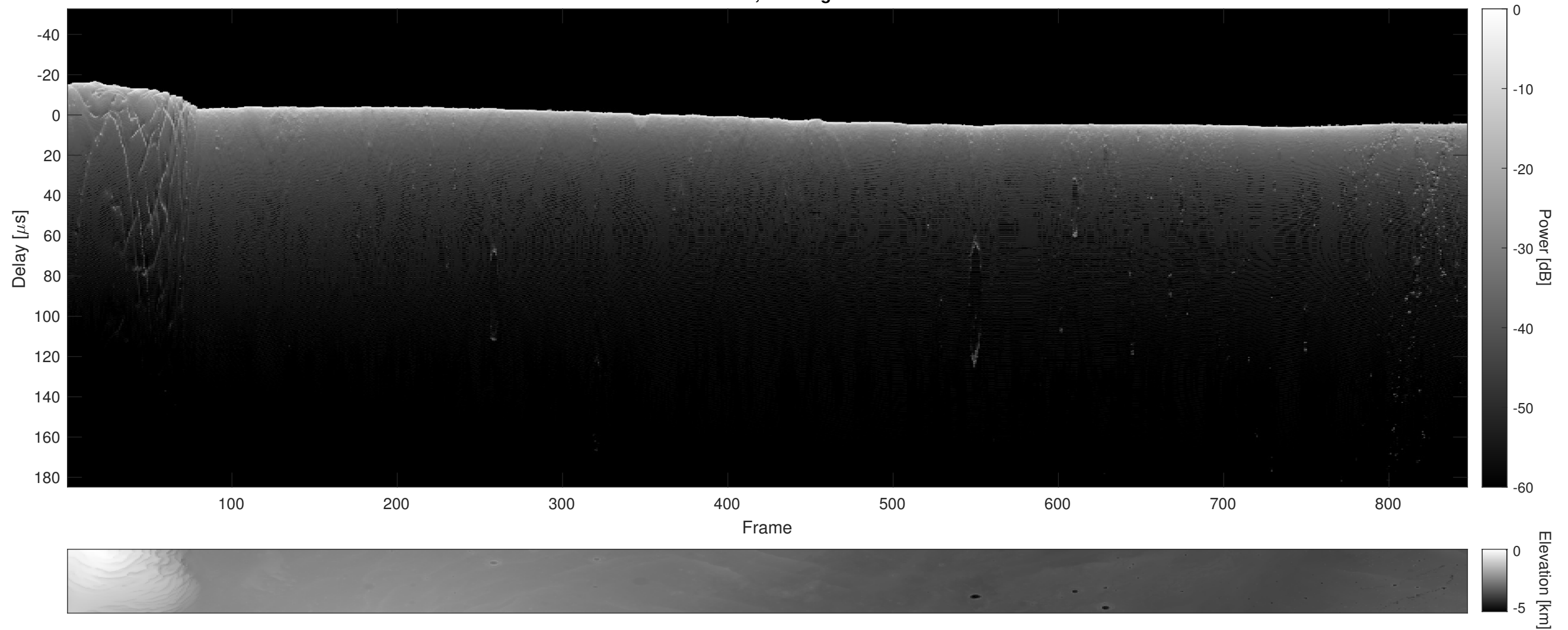
Orbit 9490, Cluttergram
