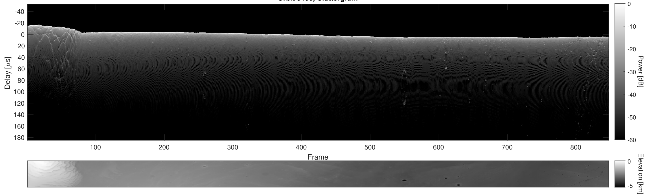
Orbit 9490, Cluttergram
