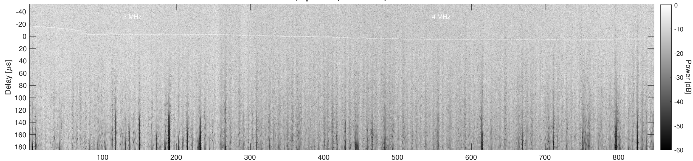
Orbit 9490, Cluttergram
