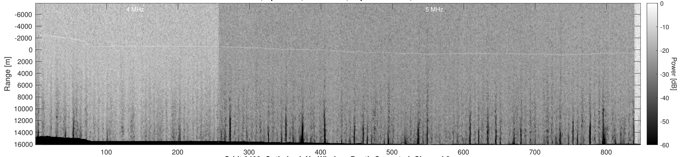
Orbit 9490, Optimized, No Window, Depth-Corrected, Channel 2
