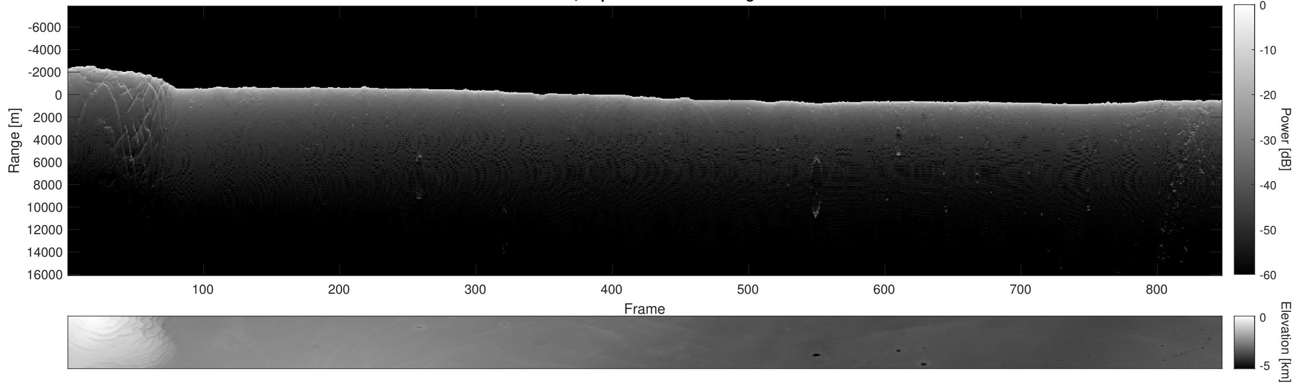
Orbit 9490, Depth-Corrected Cluttergram
