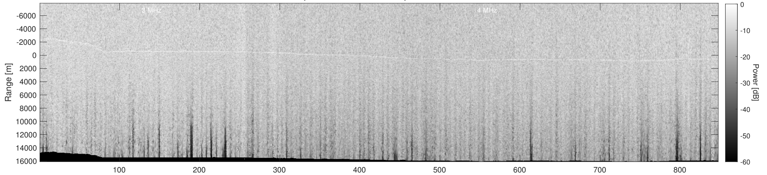
Orbit 9490, Depth-Corrected Cluttergram
