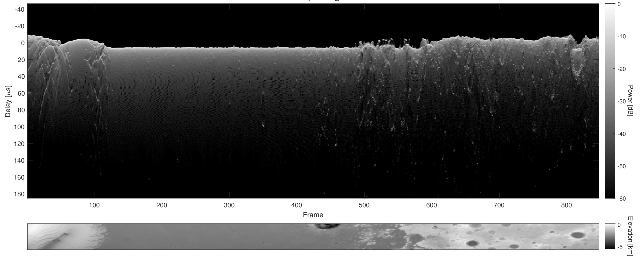
Orbit 9491, Cluttergram
