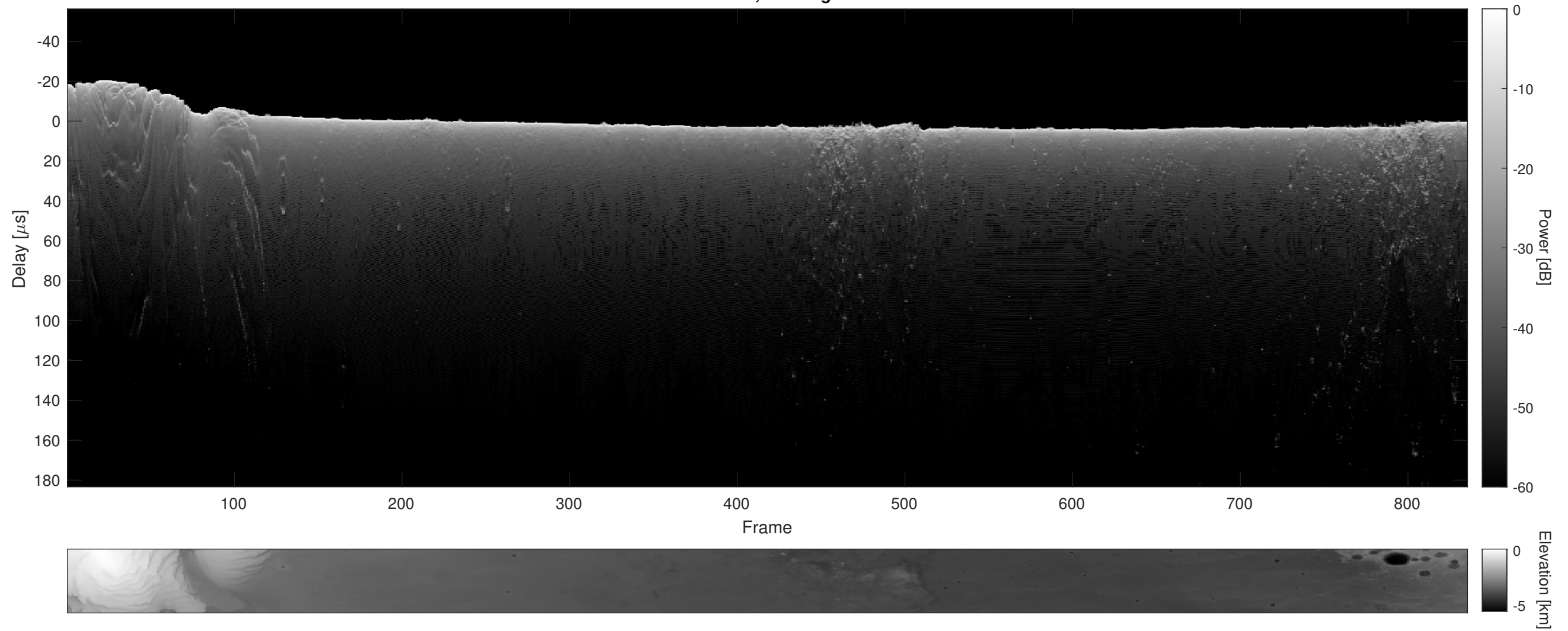
Orbit 9495, Cluttergram
