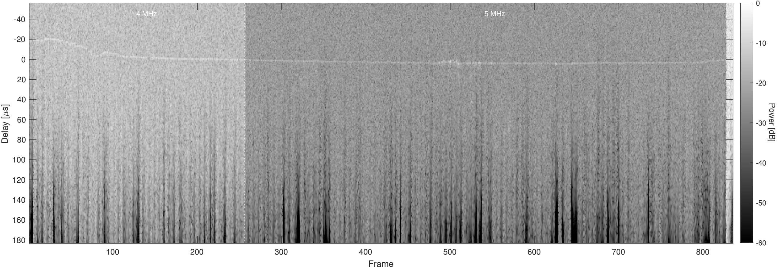
Orbit 9495, Optimized, Window, Channel 2
