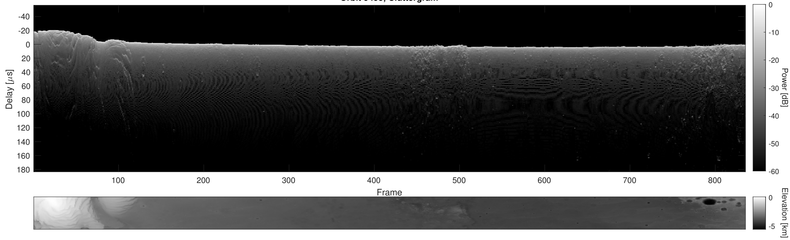
Orbit 9495, Cluttergram
