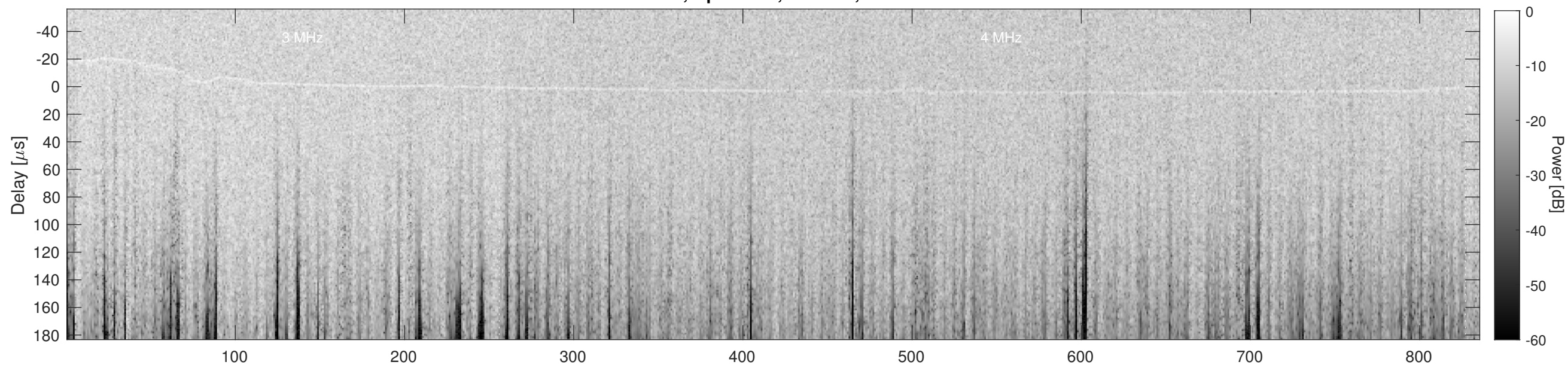
Orbit 9495, Cluttergram
