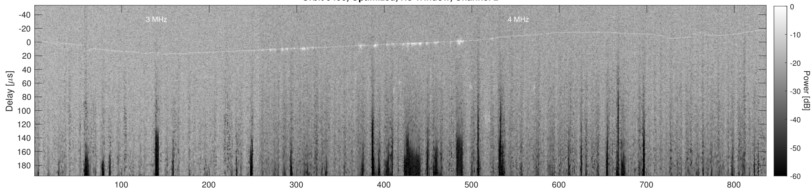
Orbit 9496, Cluttergram
