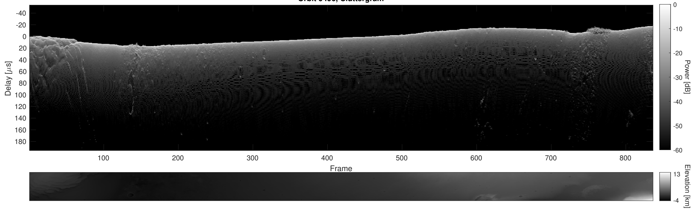
Orbit 9496, Cluttergram
