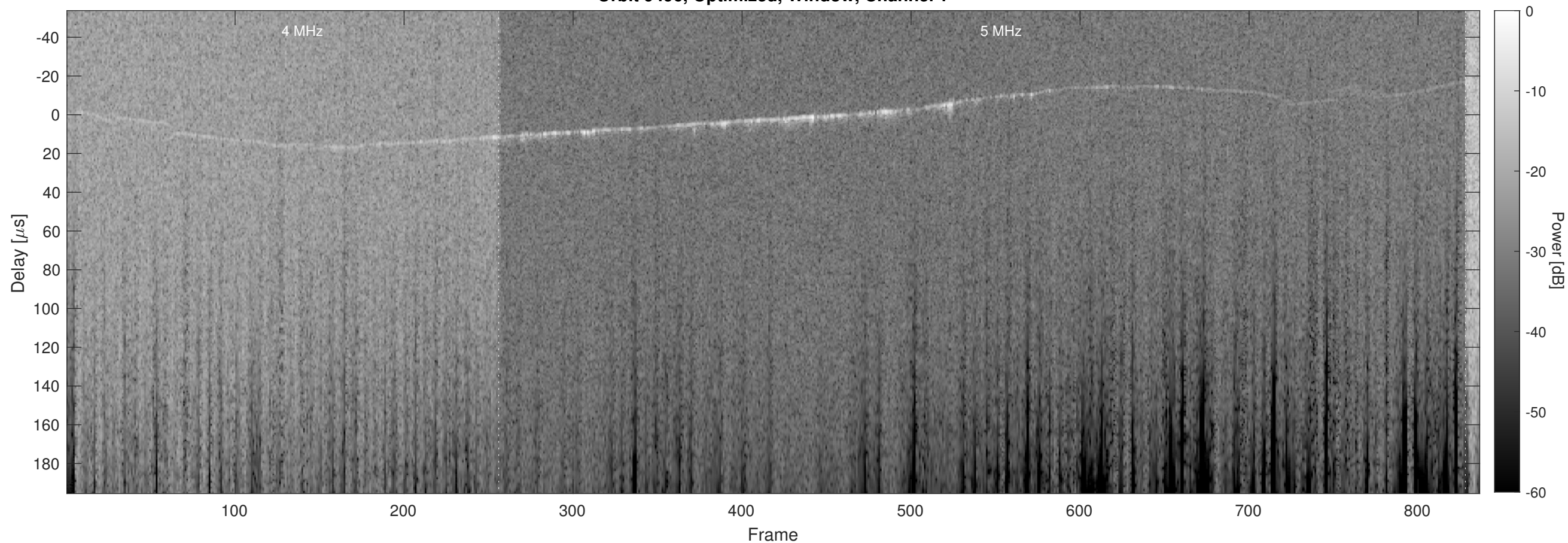
Orbit 9496, Optimized, Window, Channel 2
