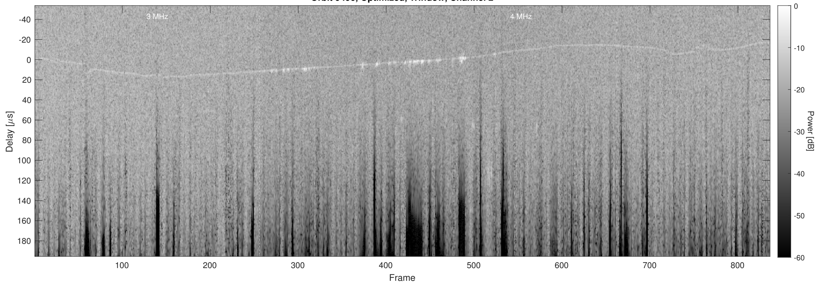
Orbit 9496, Optimized, Window, Channel 2
