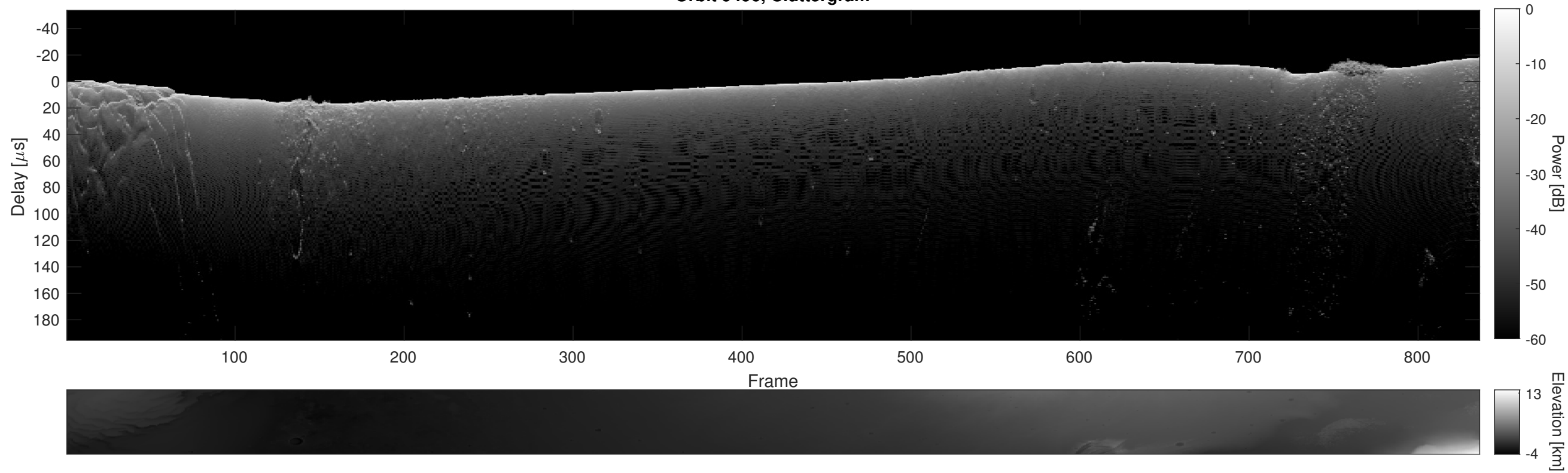
Orbit 9496, Cluttergram
