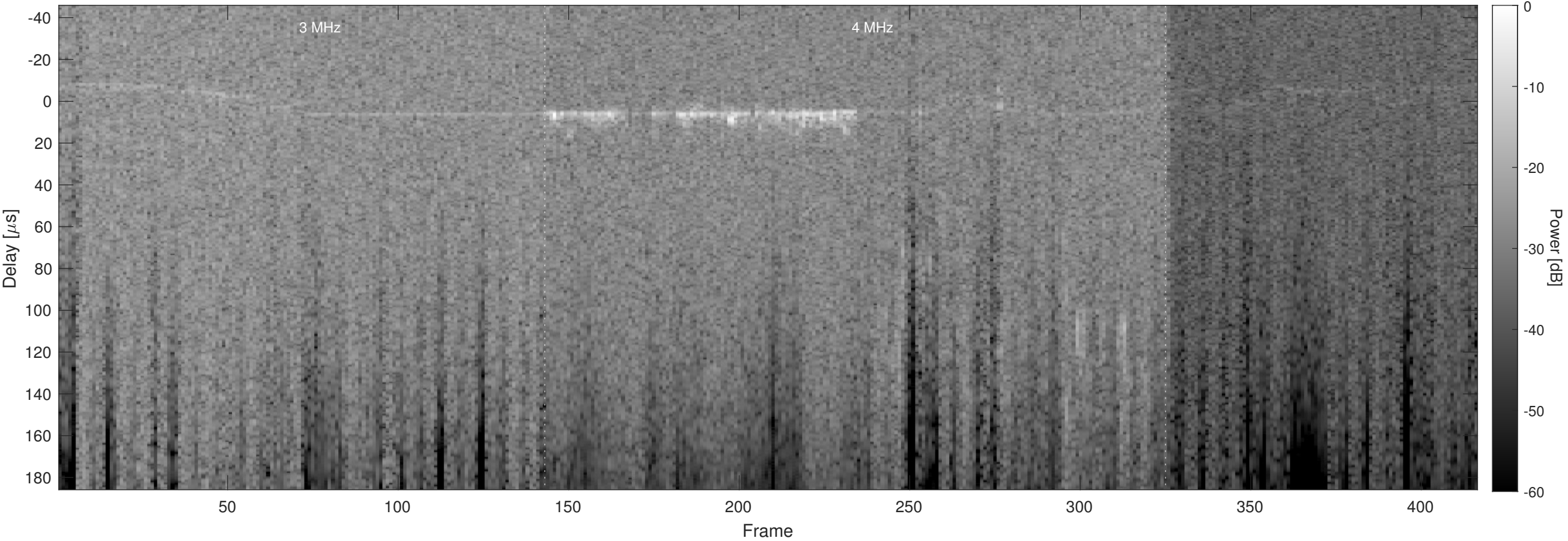
Orbit 9498, Optimized, Window, Channel 2
