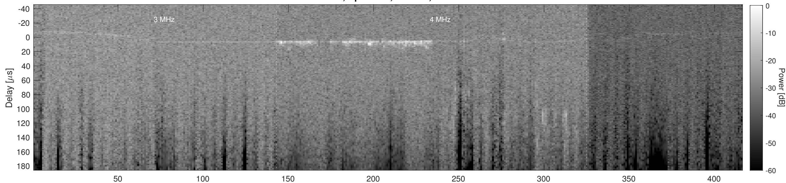
Orbit 9498, Cluttergram
