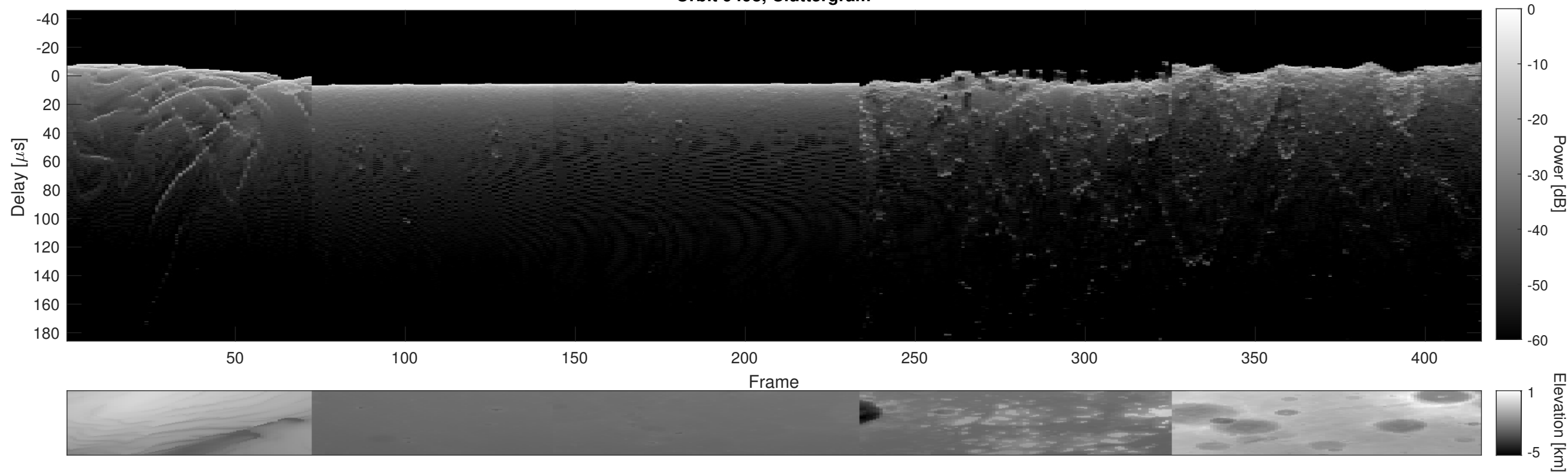
Orbit 9498, Cluttergram
