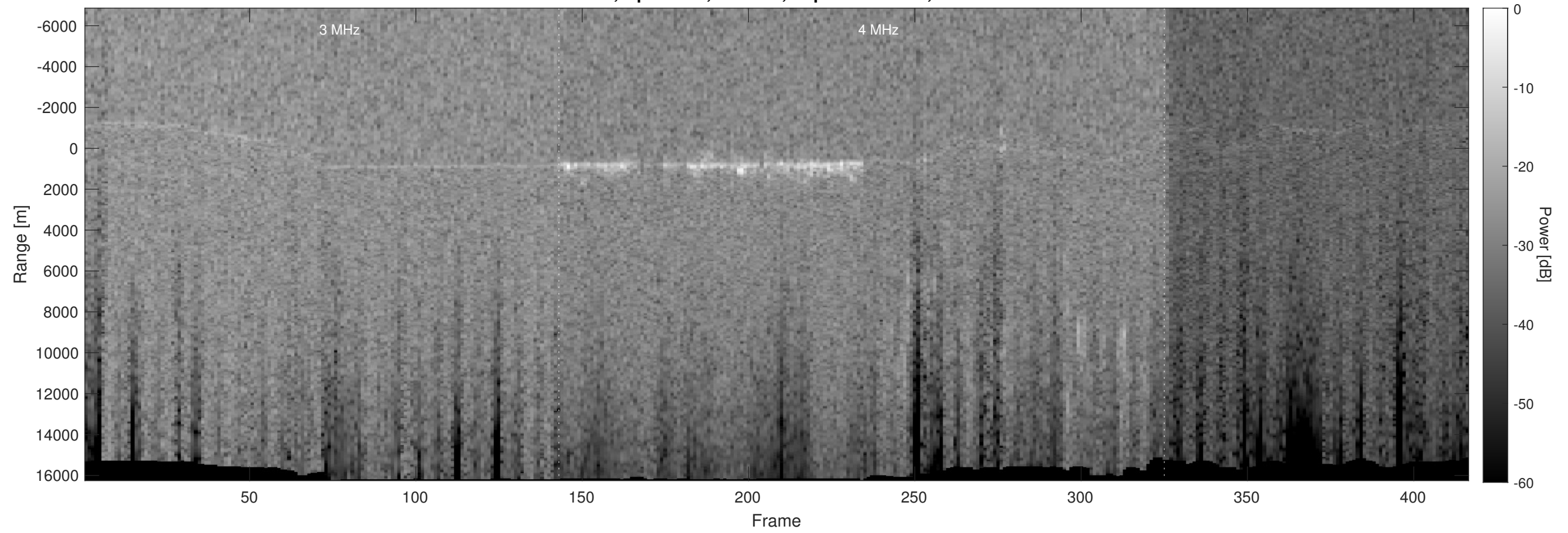
Orbit 9498, Optimized, Window, Depth-Corrected, Channel 2
