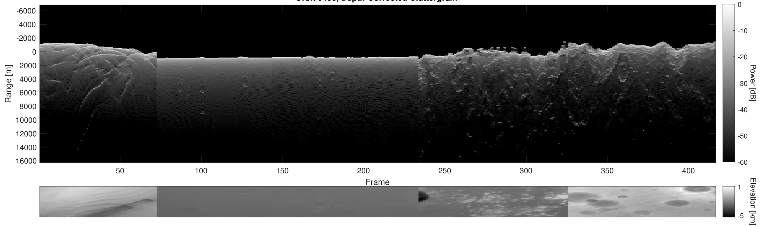
Orbit 9498, Depth-Corrected Cluttergram
