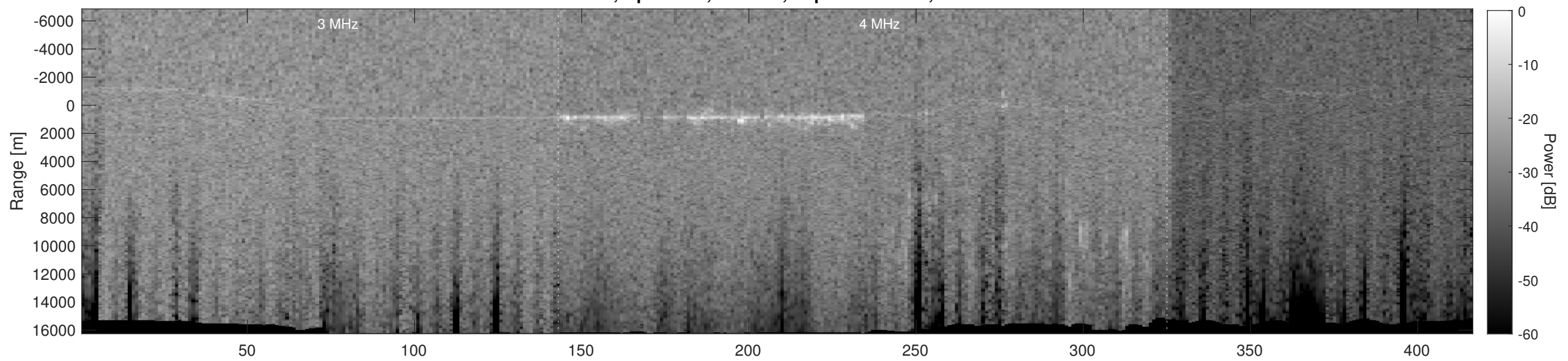
Orbit 9498, Depth-Corrected Cluttergram
