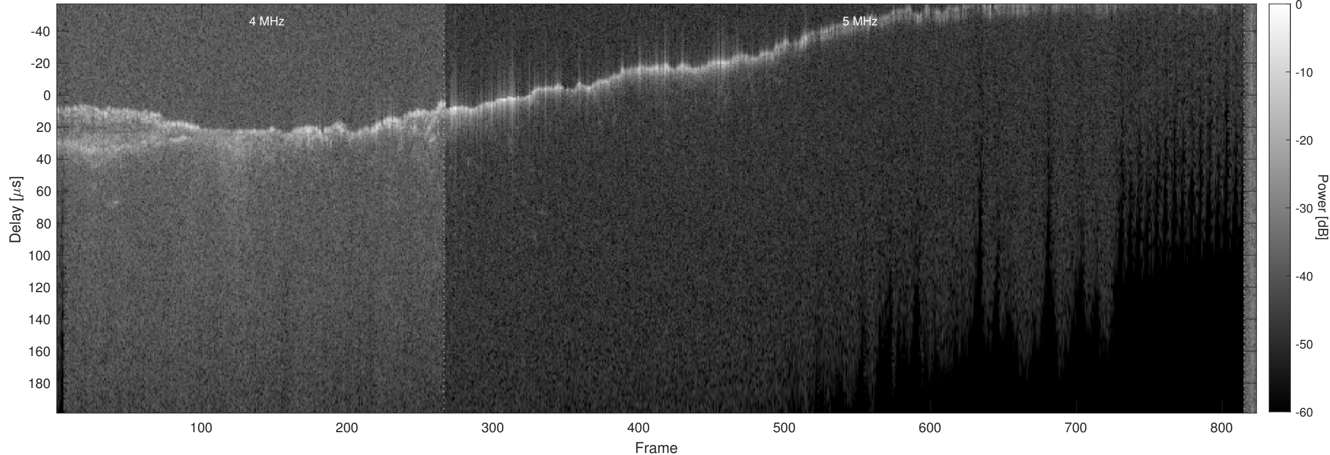
Orbit 9503, Chapman, No Window, Channel 2
