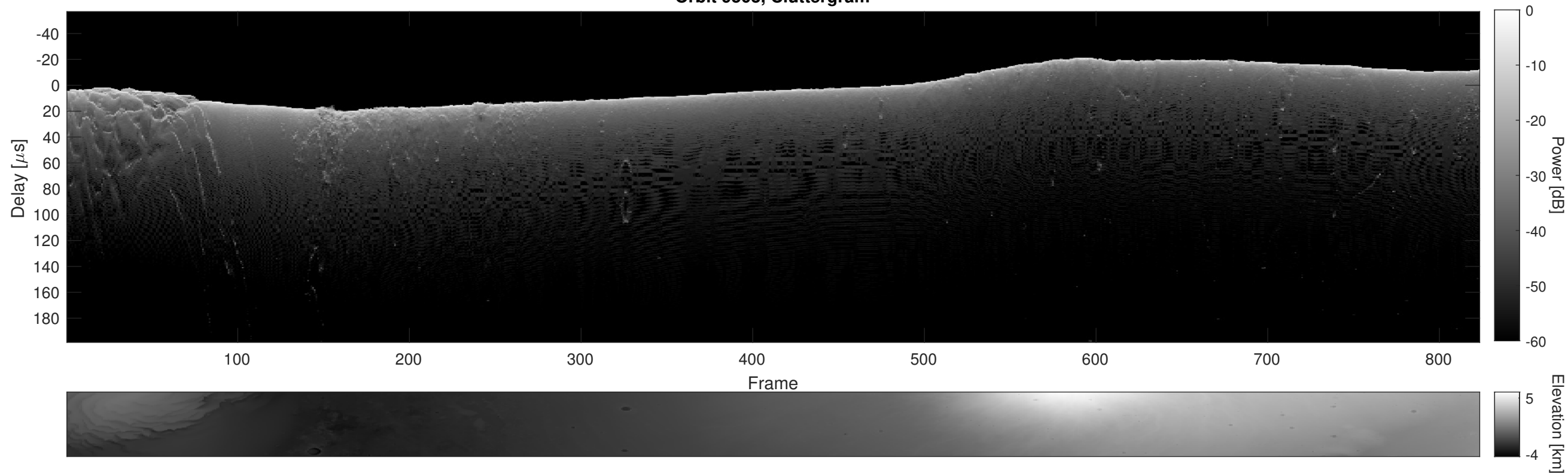
Orbit 9503, Cluttergram
