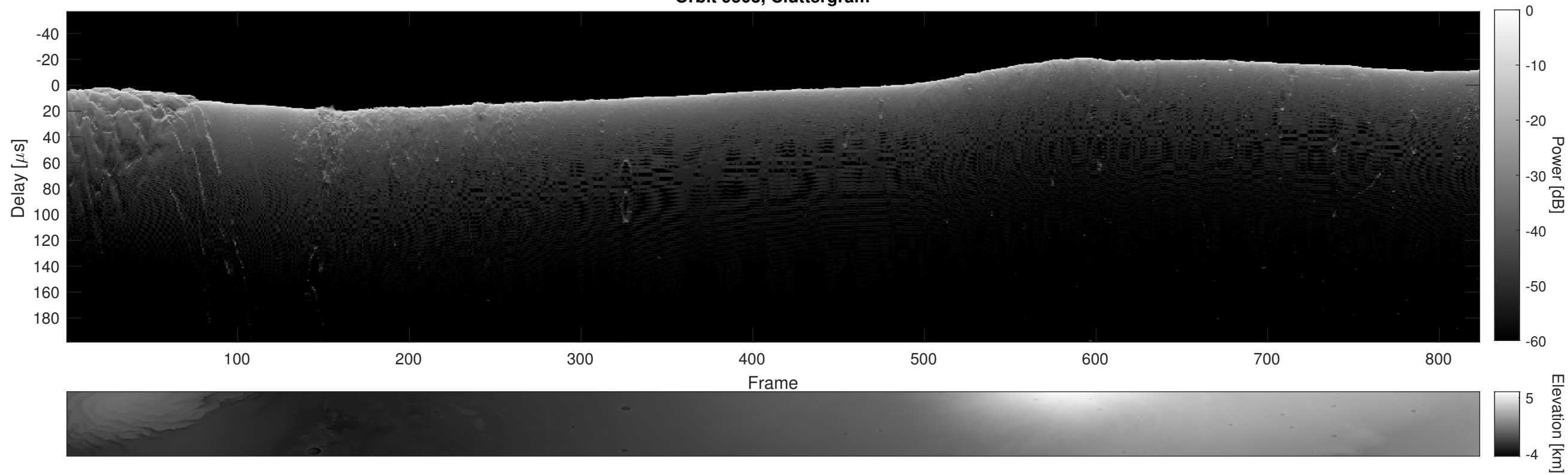
Orbit 9503, Cluttergram
