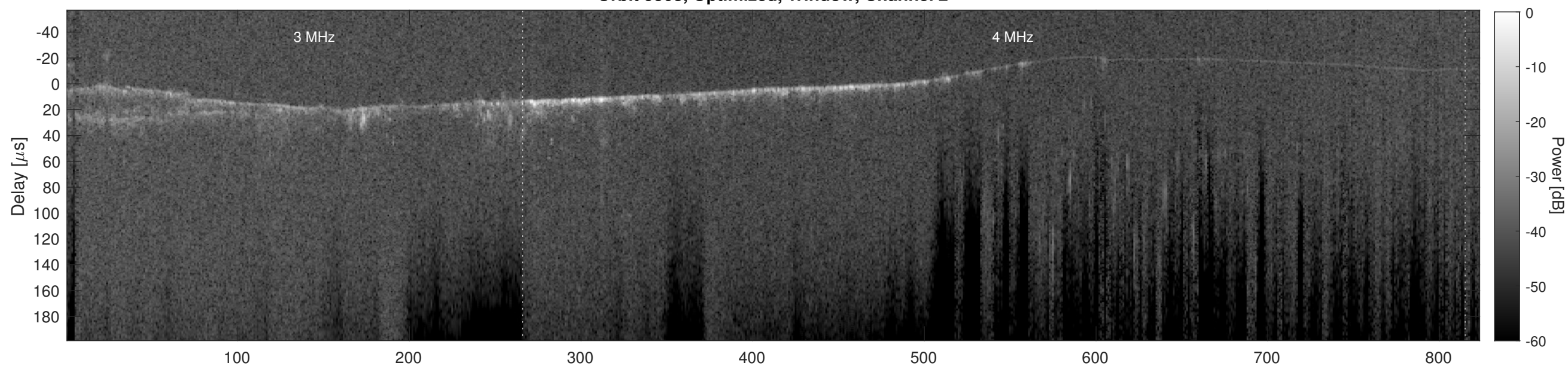
Orbit 9503, Cluttergram
