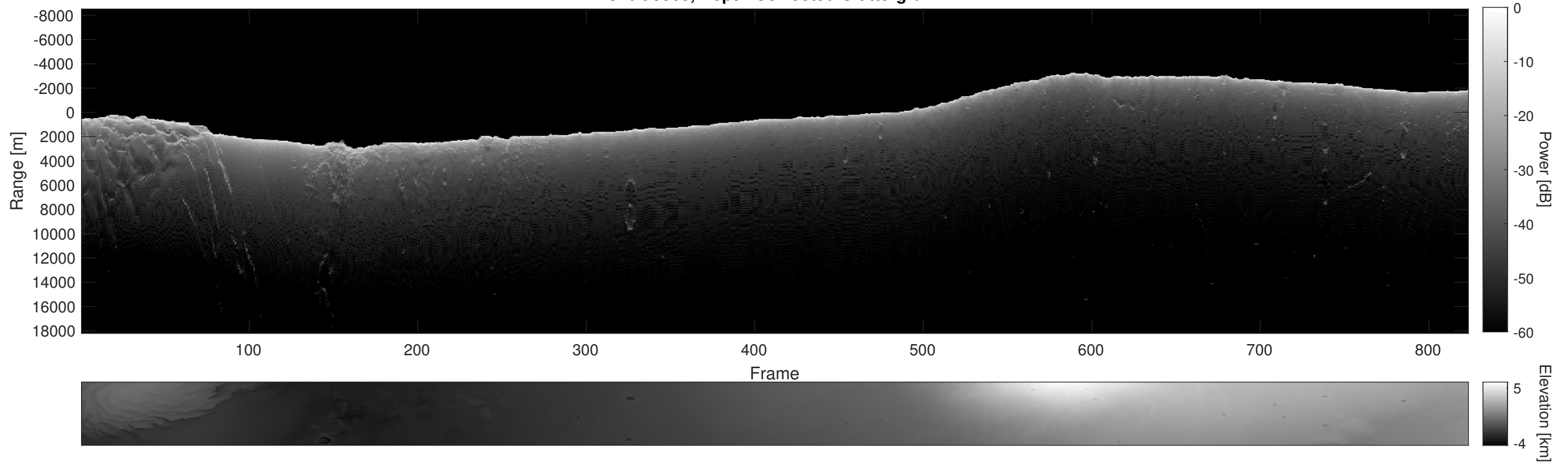
Orbit 9503, Depth-Corrected Cluttergram
