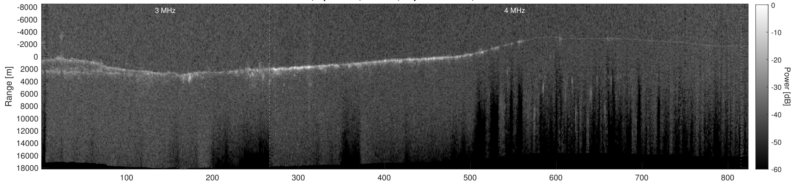
Orbit 9503, Depth-Corrected Cluttergram
